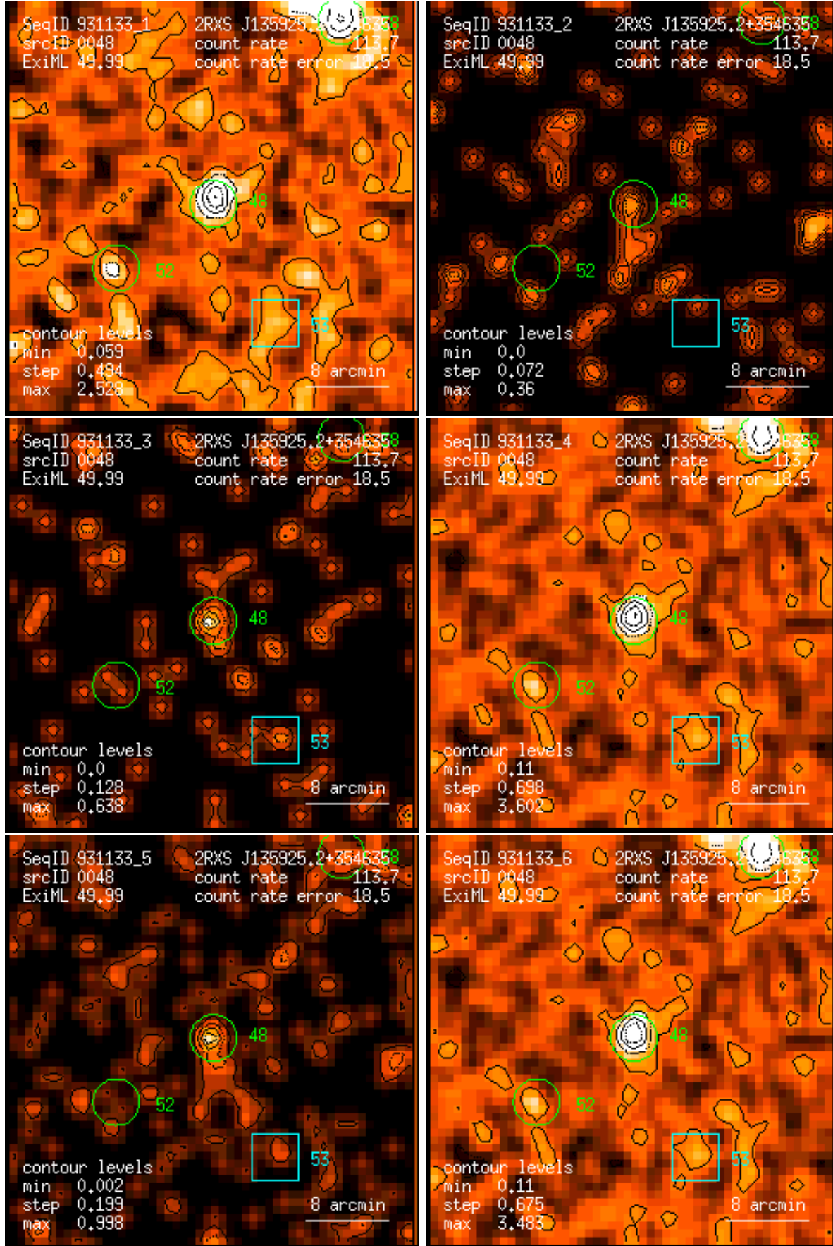
Figure 48: RASS 931133: detection 0048: band rate images, Gaussian filter: (1) PSPC channels 11 – 41, (2) 52 – 90, (3) 91 – 201, (4) 11 – 235, (5) 52 – 201, (6) 11 – 201. Broad band rates in counts/ks. Band rate contour levels in counts/ks/arcmin 2 .
