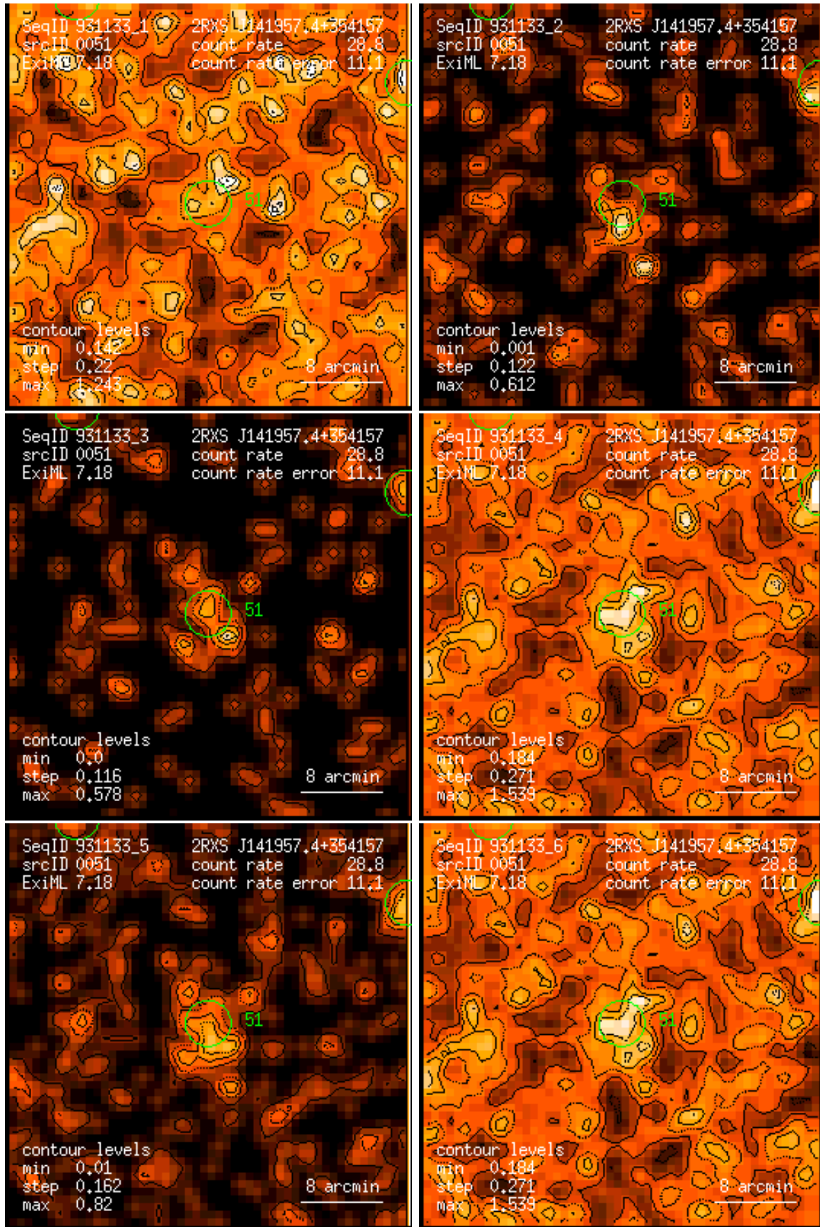
Figure 51: RASS 931133: detection 0051: band rate images, Gaussian filter: (1) PSPC channels 11 – 41, (2) 52 – 90, (3) 91 – 201, (4) 11 – 235, (5) 52 – 201, (6) 11 – 201. Broad band rates in counts/ks. Band rate contour levels in counts/ks/arcmin 2 .
