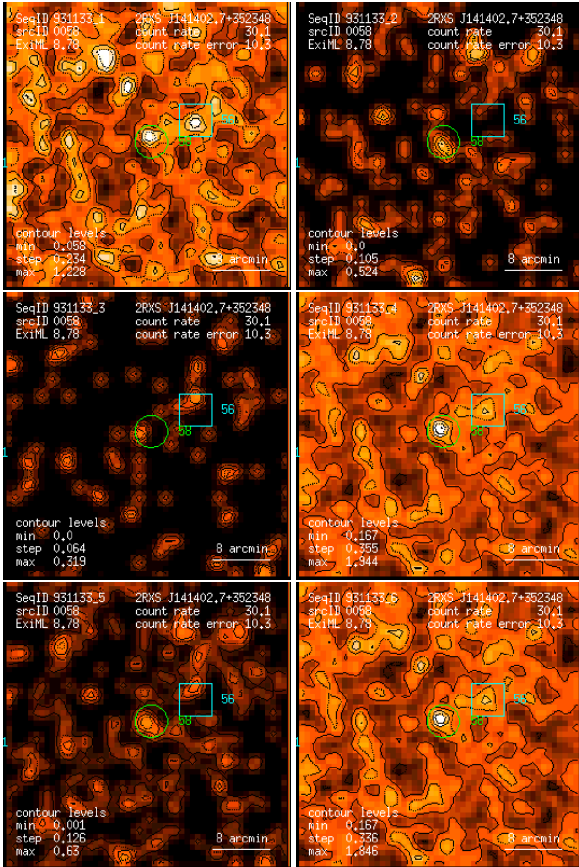
Figure 58: RASS 931133: detection 0058: band rate images, Gaussian filter: (1) PSPC channels 11 – 41, (2) 52 – 90, (3) 91 – 201, (4) 11 – 235, (5) 52 – 201, (6) 11 – 201. Broad band rates in counts/ks. Band rate contour levels in counts/ks/arcmin 2 .
