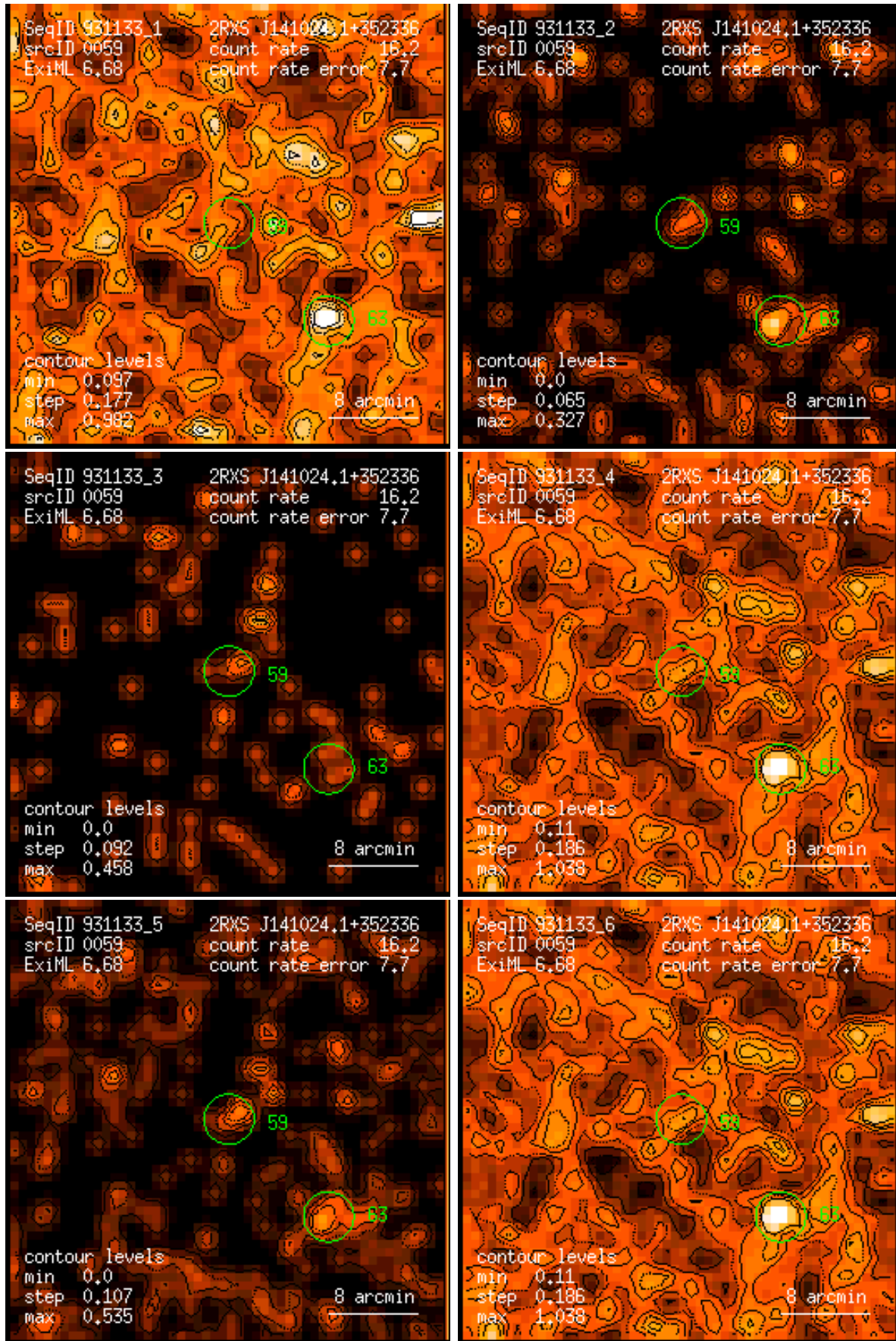
Figure 59: RASS 931133: detection 0059: band rate images, Gaussian filter: (1) PSPC channels 11 – 41, (2) 52 – 90, (3) 91 – 201, (4) 11 – 235, (5) 52 – 201, (6) 11 – 201. Broad band rates in counts/ks. Band rate contour levels in counts/ks/arcmin 2 .
