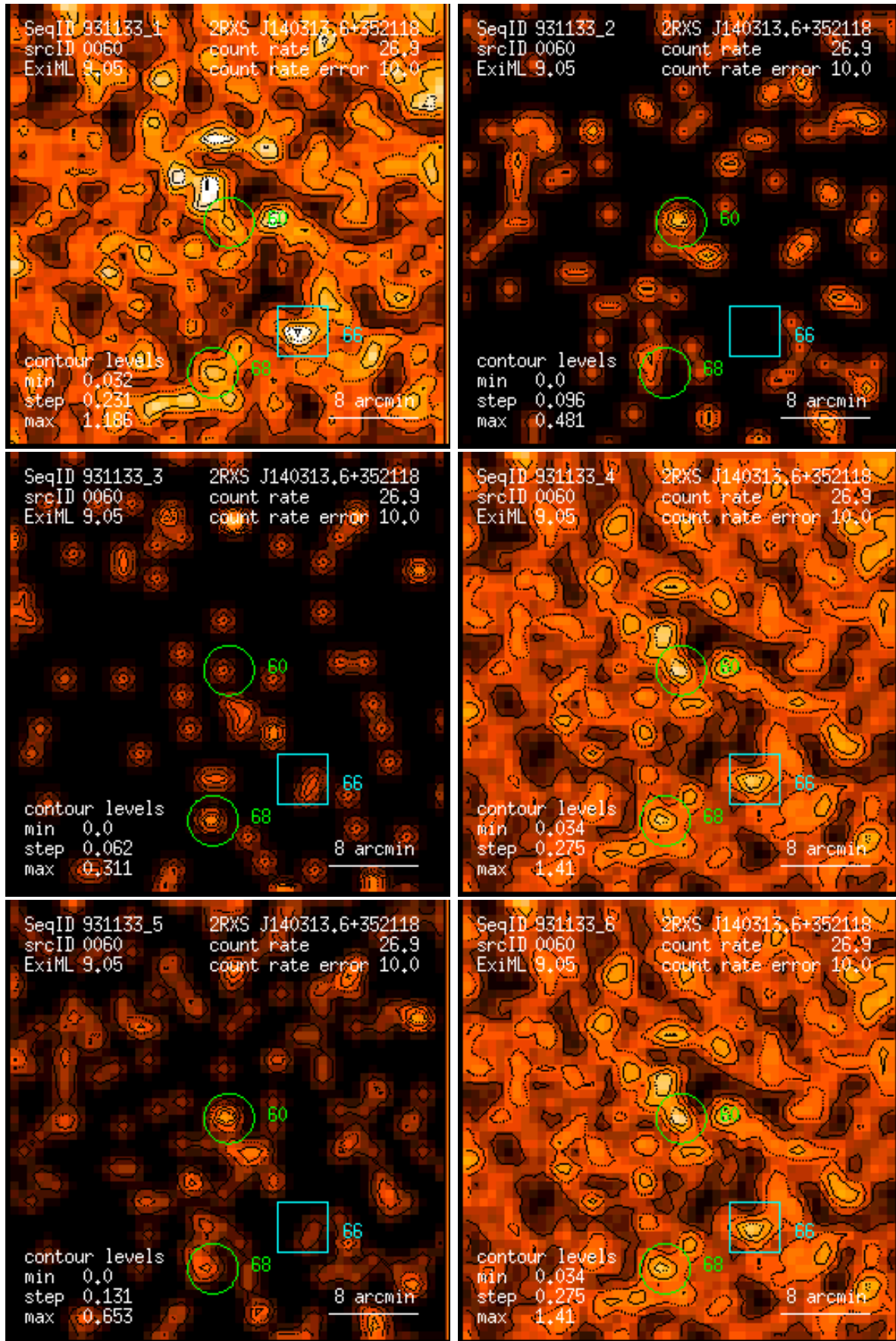
Figure 60: RASS 931133: detection 0060: band rate images, Gaussian filter: (1) PSPC channels 11 – 41, (2) 52 – 90, (3) 91 – 201, (4) 11 – 235, (5) 52 – 201, (6) 11 – 201. Broad band rates in counts/ks. Band rate contour levels in counts/ks/arcmin 2 .
