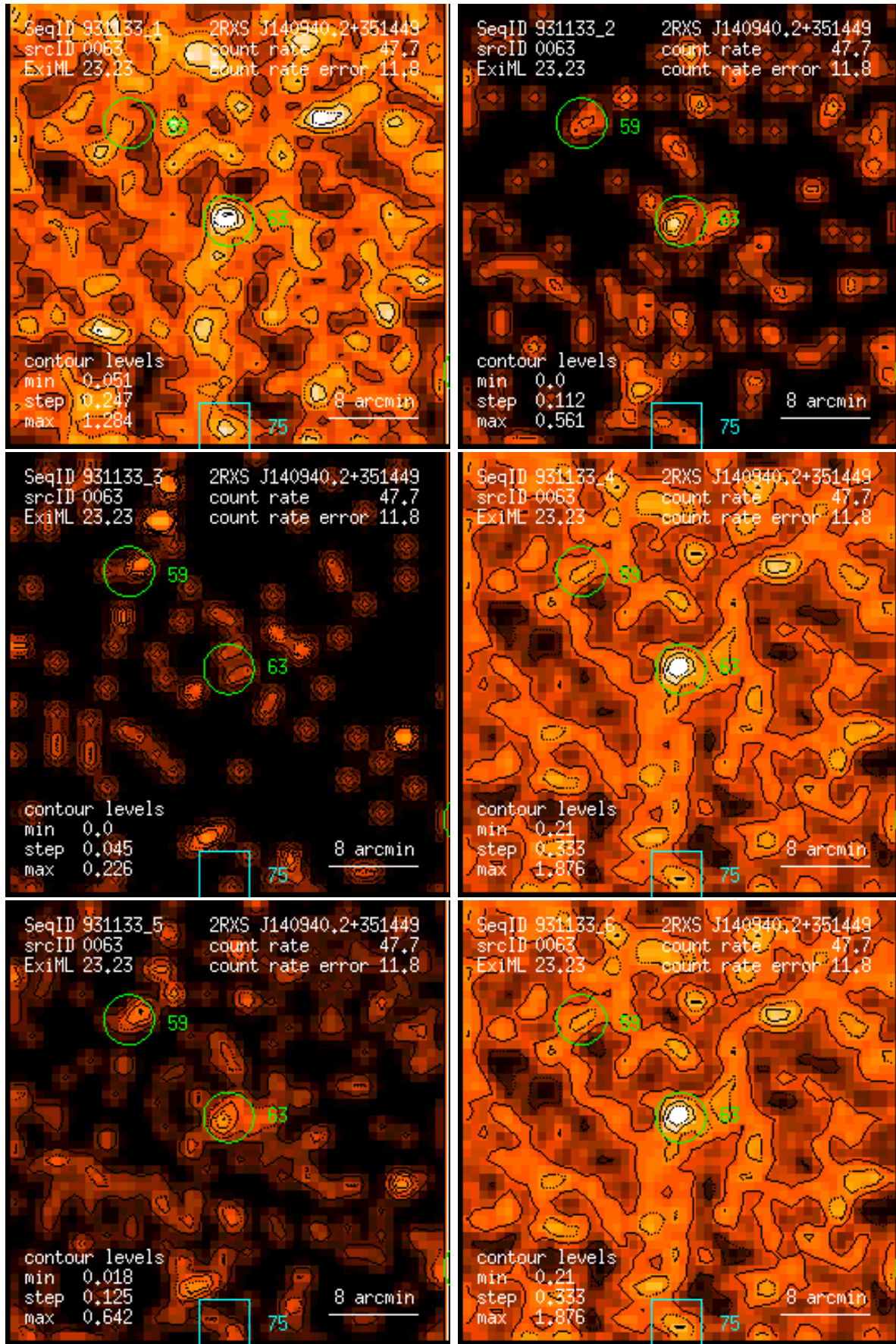
Figure 63: RASS 931133: detection 0063: band rate images, Gaussian filter: (1) PSPC channels 11 – 41, (2) 52 – 90, (3) 91 – 201, (4) 11 – 235, (5) 52 – 201, (6) 11 – 201. Broad band rates in counts/ks. Band rate contour levels in counts/ks/arcmin 2 .
