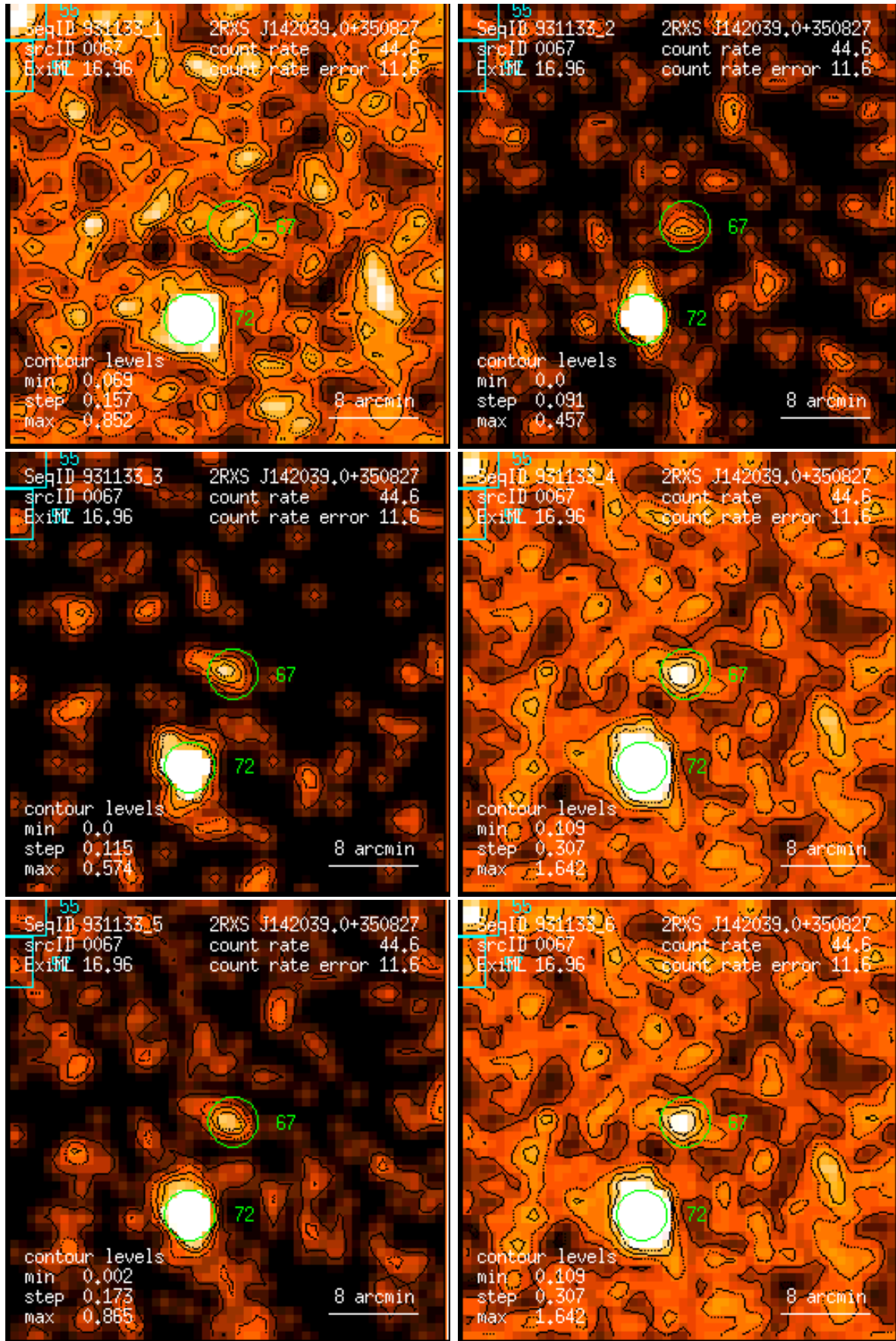
Figure 67: RASS 931133: detection 0067: band rate images, Gaussian filter: (1) PSPC channels 11 – 41, (2) 52 – 90, (3) 91 – 201, (4) 11 – 235, (5) 52 – 201, (6) 11 – 201. Broad band rates in counts/ks. Band rate contour levels in counts/ks/arcmin 2 .
