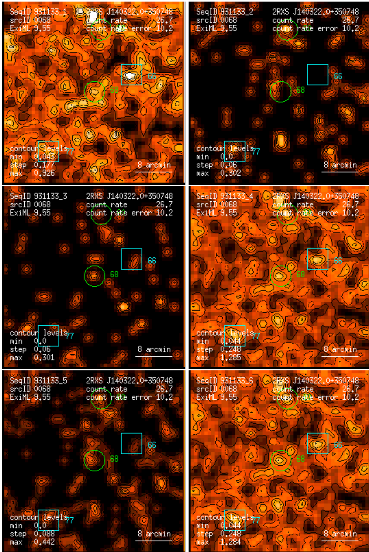
Figure 68: RASS 931133: detection 0068: band rate images, Gaussian filter: (1) PSPC channels 11 – 41, (2) 52 – 90, (3) 91 – 201, (4) 11 – 235, (5) 52 – 201, (6) 11 – 201. Broad band rates in counts/ks. Band rate contour levels in counts/ks/arcmin 2 .
