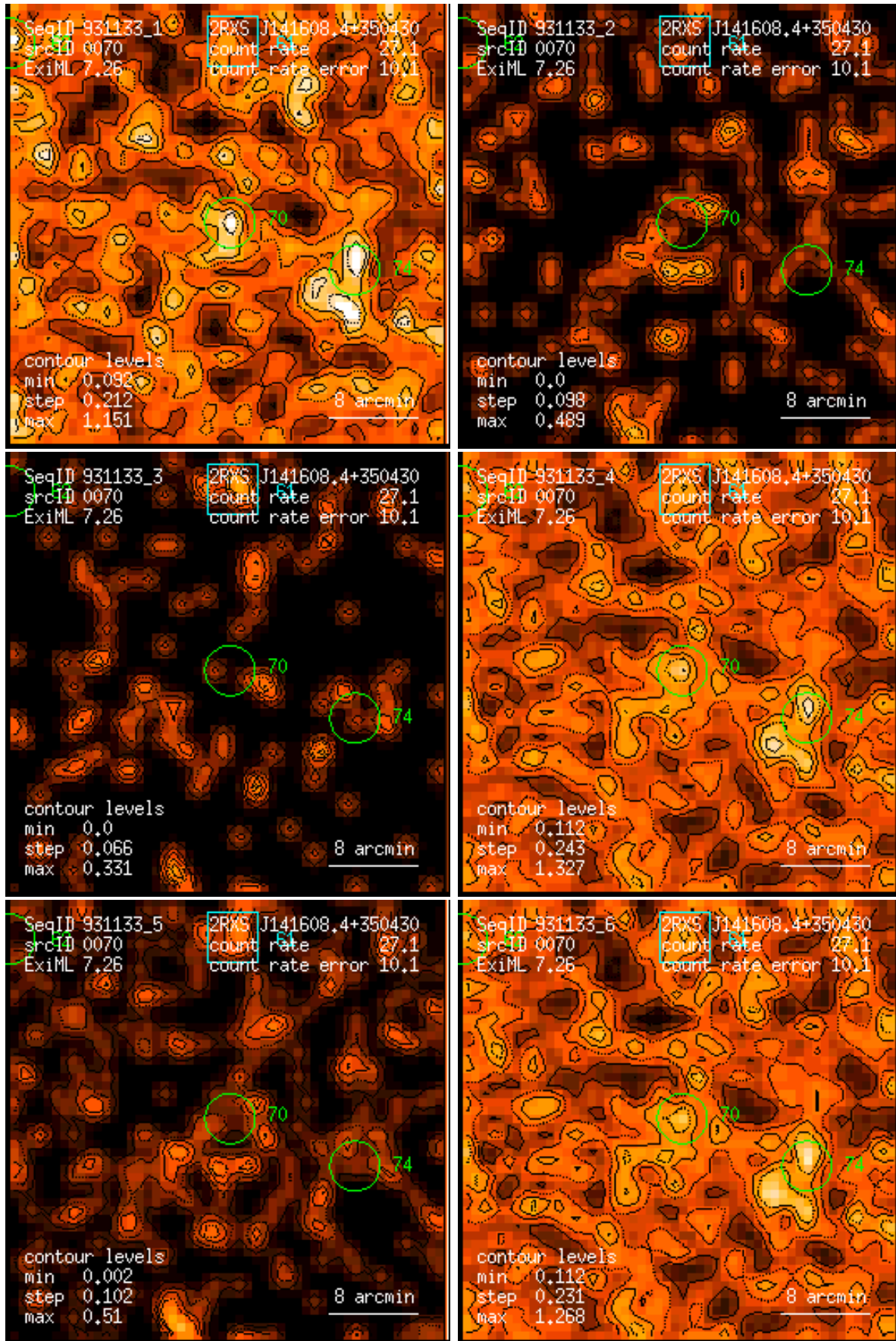
Figure 70: RASS 931133: detection 0070: band rate images, Gaussian filter: (1) PSPC channels 11 – 41, (2) 52 – 90, (3) 91 – 201, (4) 11 – 235, (5) 52 – 201, (6) 11 – 201. Broad band rates in counts/ks. Band rate contour levels in counts/ks/arcmin 2 .
