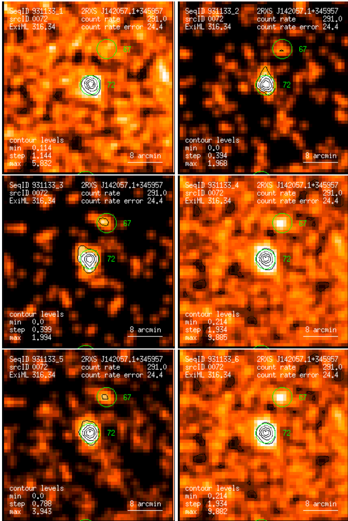
Figure 72: RASS 931133: detection 0072: band rate images, Gaussian filter: (1) PSPC channels 11 – 41, (2) 52 – 90, (3) 91 – 201, (4) 11 – 235, (5) 52 – 201, (6) 11 – 201. Broad band rates in counts/ks. Band rate contour levels in counts/ks/arcmin 2 .
