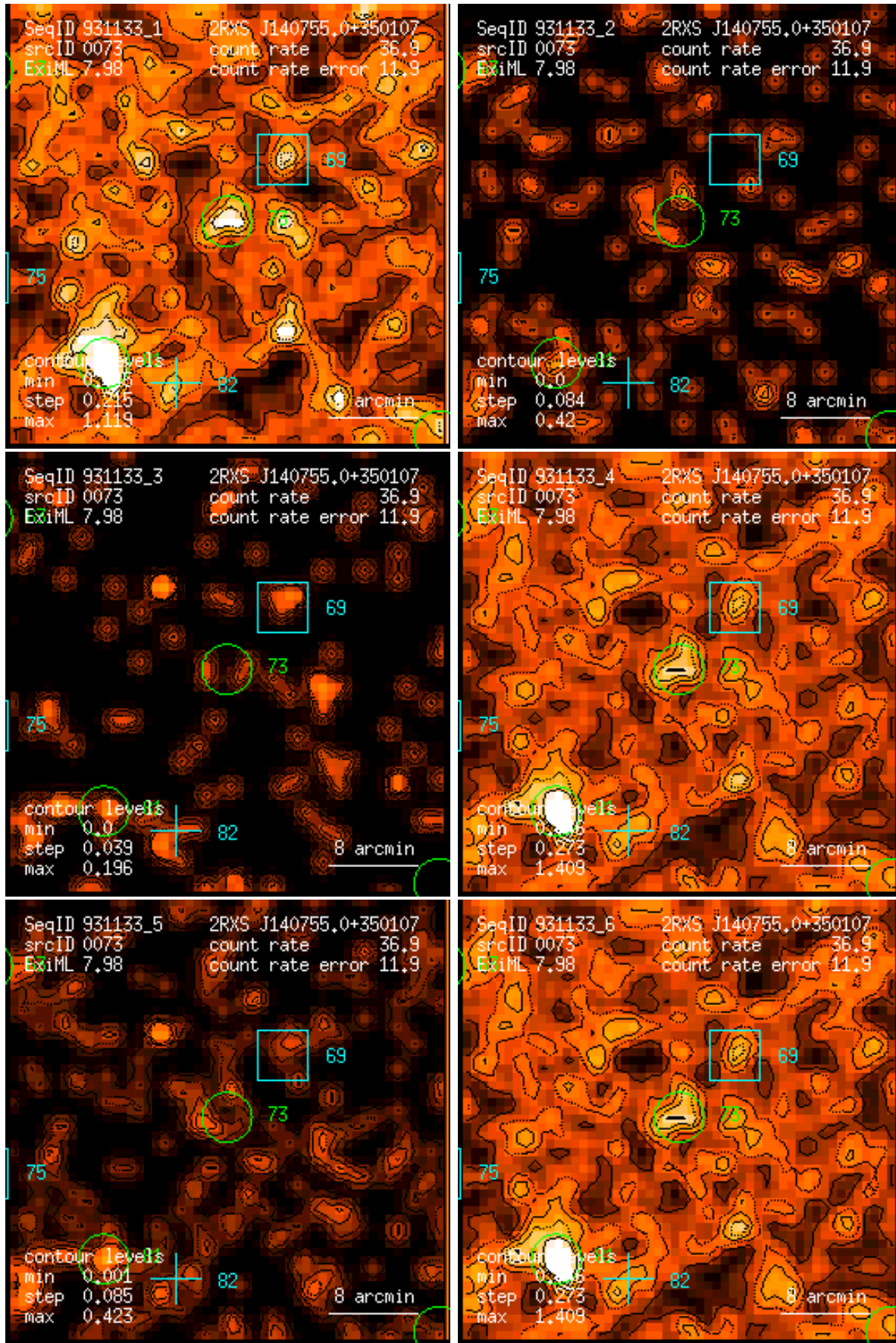
Figure 73: RASS 931133: detection 0073: band rate images, Gaussian filter: (1) PSPC channels 11 – 41, (2) 52 – 90, (3) 91 – 201, (4) 11 – 235, (5) 52 – 201, (6) 11 – 201. Broad band rates in counts/ks. Band rate contour levels in counts/ks/arcmin 2 .
