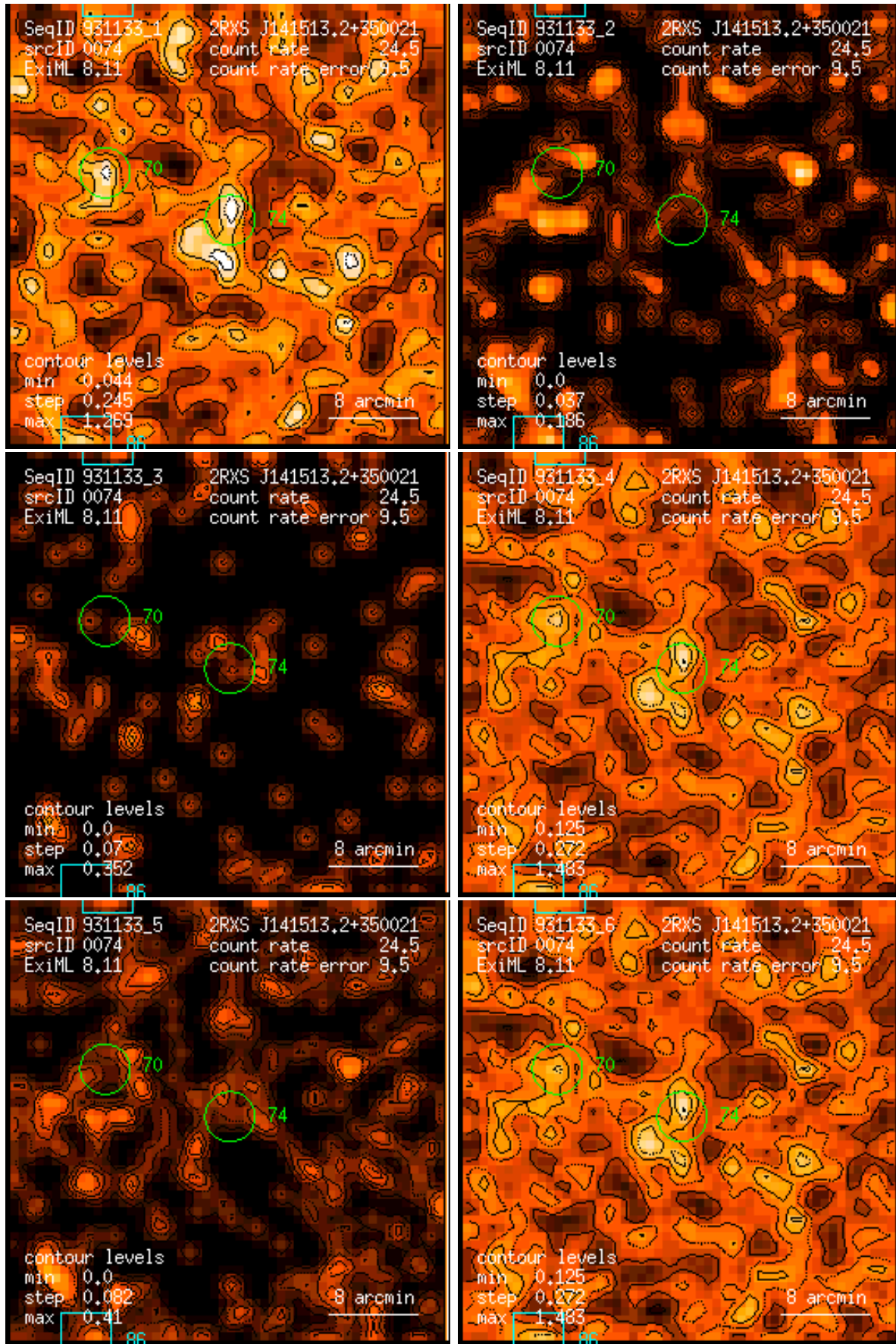
Figure 74: RASS 931133: detection 0074: band rate images, Gaussian filter: (1) PSPC channels 11 – 41, (2) 52 – 90, (3) 91 – 201, (4) 11 – 235, (5) 52 – 201, (6) 11 – 201. Broad band rates in counts/ks. Band rate contour levels in counts/ks/arcmin 2 .
