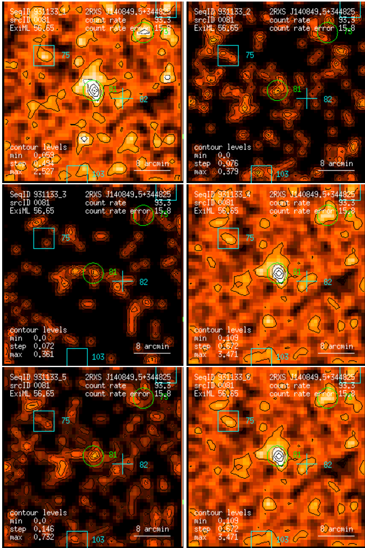
Figure 81: RASS 931133: detection 0081: band rate images, Gaussian filter: (1) PSPC channels 11 – 41, (2) 52 – 90, (3) 91 – 201, (4) 11 – 235, (5) 52 – 201, (6) 11 – 201. Broad band rates in counts/ks. Band rate contour levels in counts/ks/arcmin 2 .
