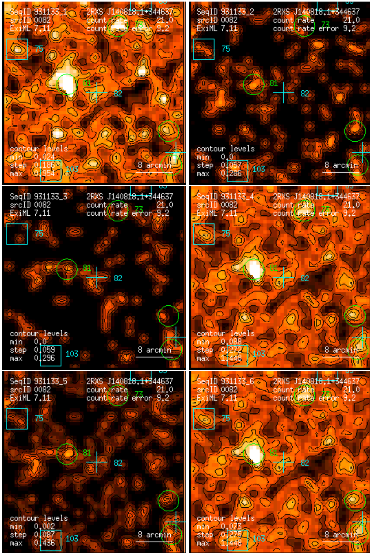
Figure 82: RASS 931133: detection 0082: band rate images, Gaussian filter: (1) PSPC channels 11 – 41, (2) 52 – 90, (3) 91 – 201, (4) 11 – 235, (5) 52 – 201, (6) 11 – 201. Broad band rates in counts/ks. Band rate contour levels in counts/ks/arcmin 2 .
