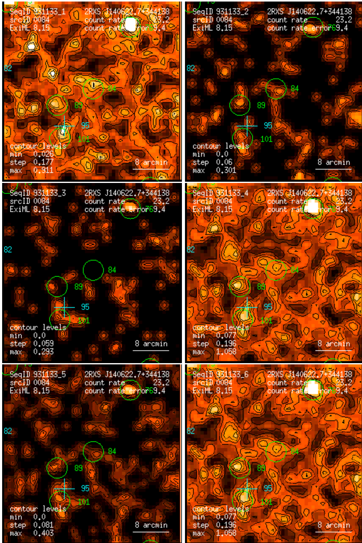
Figure 84: RASS 931133: detection 0084: band rate images, Gaussian filter: (1) PSPC channels 11 – 41, (2) 52 – 90, (3) 91 – 201, (4) 11 – 235, (5) 52 – 201, (6) 11 – 201. Broad band rates in counts/ks. Band rate contour levels in counts/ks/arcmin 2 .
