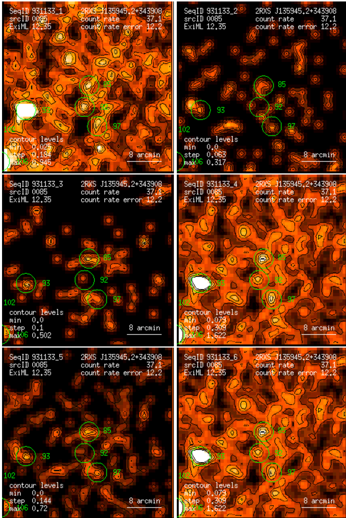
Figure 85: RASS 931133: detection 0085: band rate images, Gaussian filter: (1) PSPC channels 11 – 41, (2) 52 – 90, (3) 91 – 201, (4) 11 – 235, (5) 52 – 201, (6) 11 – 201. Broad band rates in counts/ks. Band rate contour levels in counts/ks/arcmin 2 .
