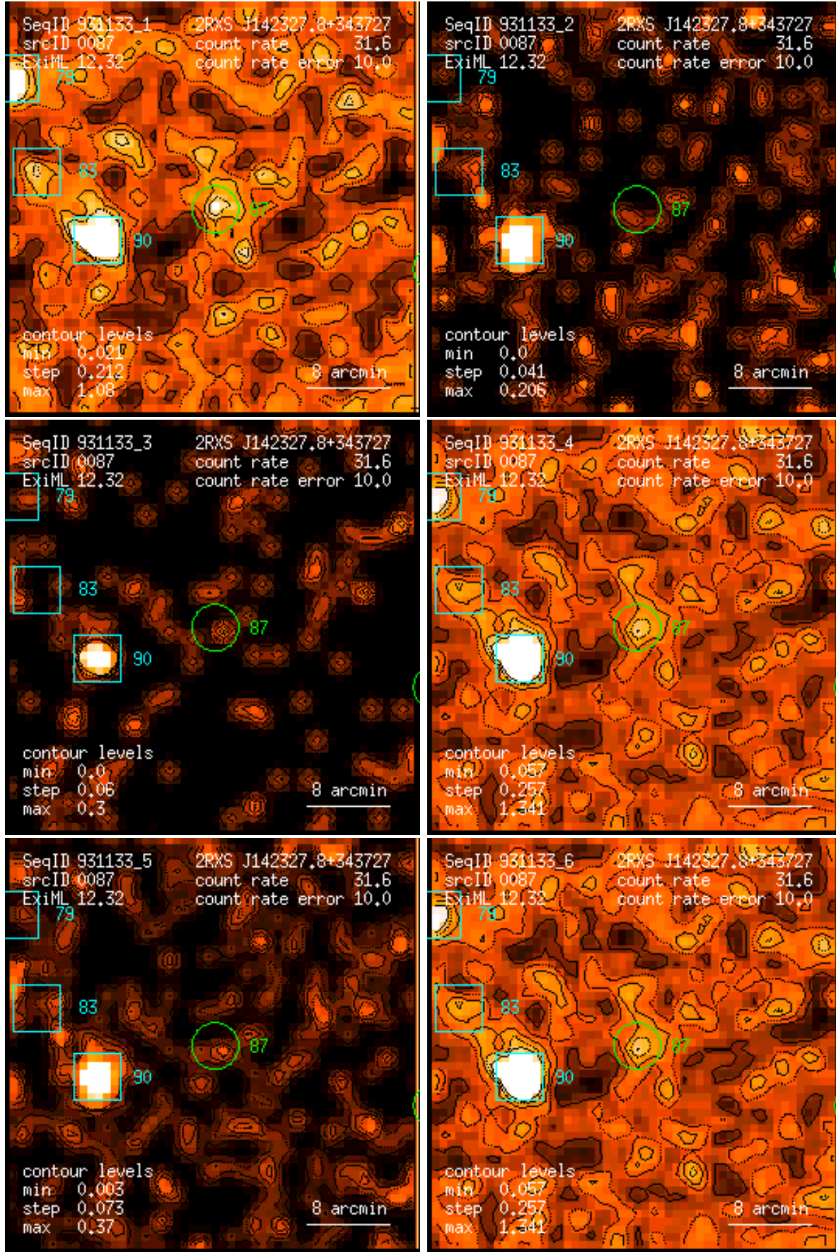
Figure 87: RASS 931133: detection 0087: band rate images, Gaussian filter: (1) PSPC channels 11 – 41, (2) 52 – 90, (3) 91 – 201, (4) 11 – 235, (5) 52 – 201, (6) 11 – 201. Broad band rates in counts/ks. Band rate contour levels in counts/ks/arcmin 2 .
