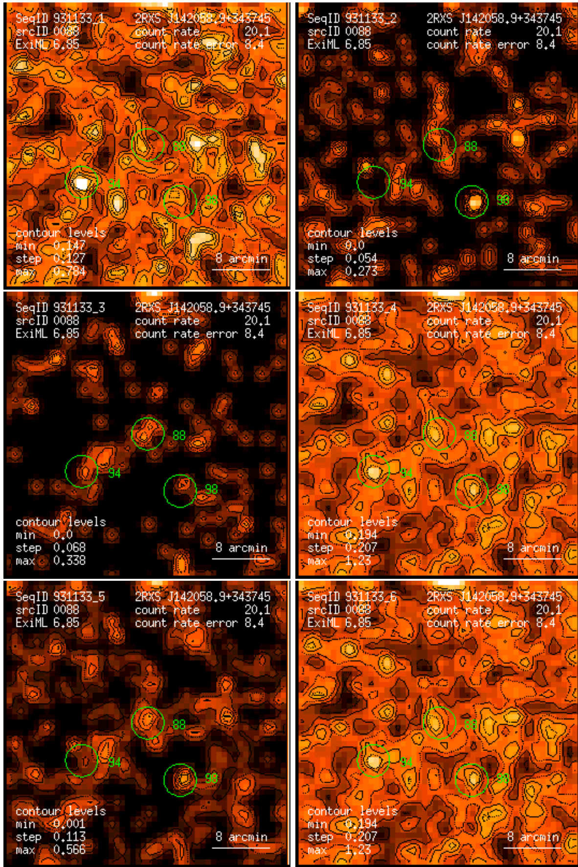
Figure 88: RASS 931133: detection 0088: band rate images, Gaussian filter: (1) PSPC channels 11 – 41, (2) 52 – 90, (3) 91 – 201, (4) 11 – 235, (5) 52 – 201, (6) 11 – 201. Broad band rates in counts/ks. Band rate contour levels in counts/ks/arcmin 2 .
