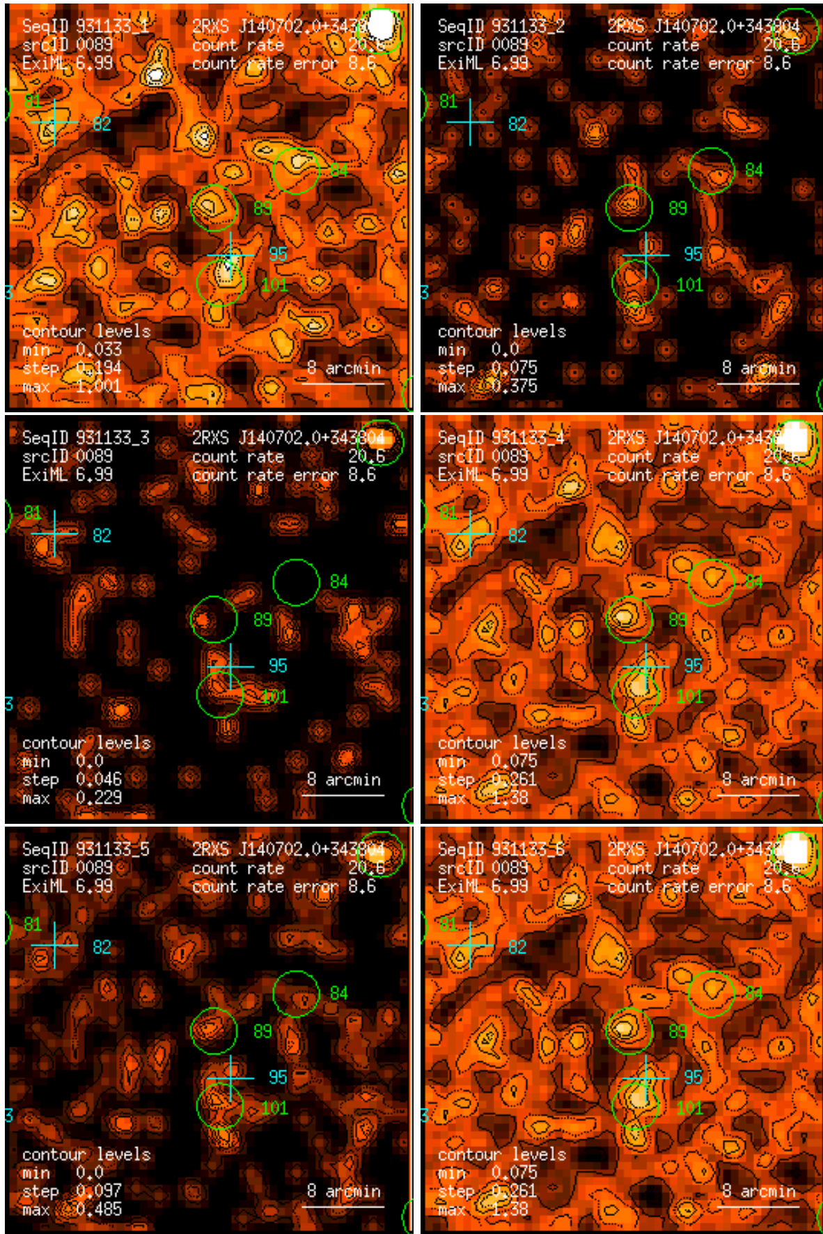
Figure 89: RASS 931133: detection 0089: band rate images, Gaussian filter: (1) PSPC channels 11 – 41, (2) 52 – 90, (3) 91 – 201, (4) 11 – 235, (5) 52 – 201, (6) 11 – 201. Broad band rates in counts/ks. Band rate contour levels in counts/ks/arcmin 2 .
