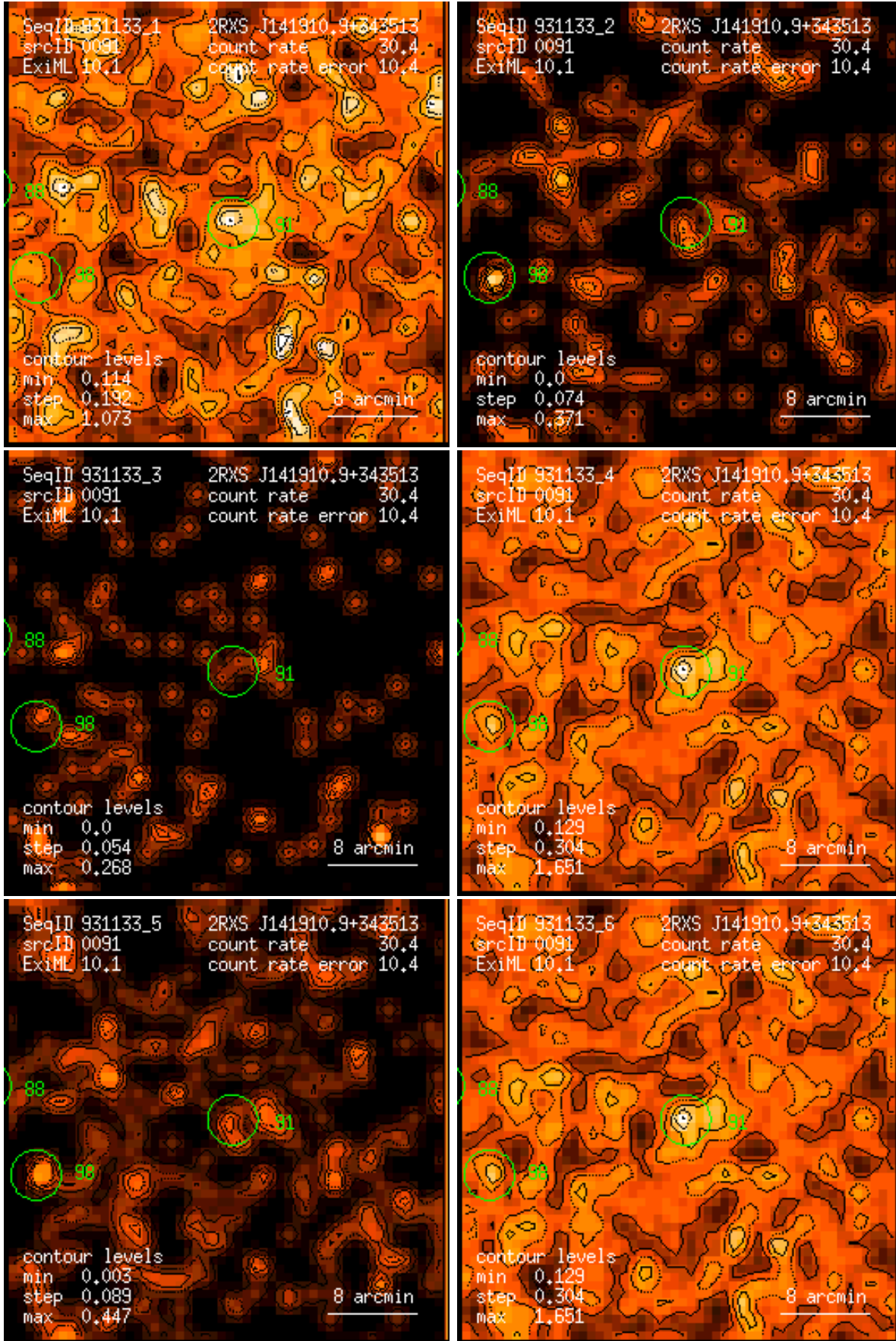
Figure 91: RASS 931133: detection 0091: band rate images, Gaussian filter: (1) PSPC channels 11 – 41, (2) 52 – 90, (3) 91 – 201, (4) 11 – 235, (5) 52 – 201, (6) 11 – 201. Broad band rates in counts/ks. Band rate contour levels in counts/ks/arcmin 2 .
