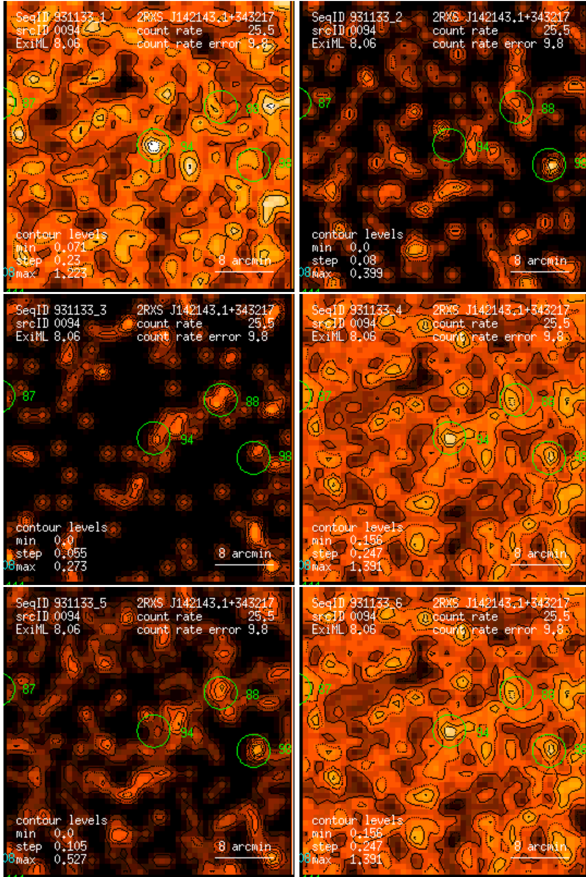
Figure 94: RASS 931133: detection 0094: band rate images, Gaussian filter: (1) PSPC channels 11 – 41, (2) 52 – 90, (3) 91 – 201, (4) 11 – 235, (5) 52 – 201, (6) 11 – 201. Broad band rates in counts/ks. Band rate contour levels in counts/ks/arcmin 2 .
