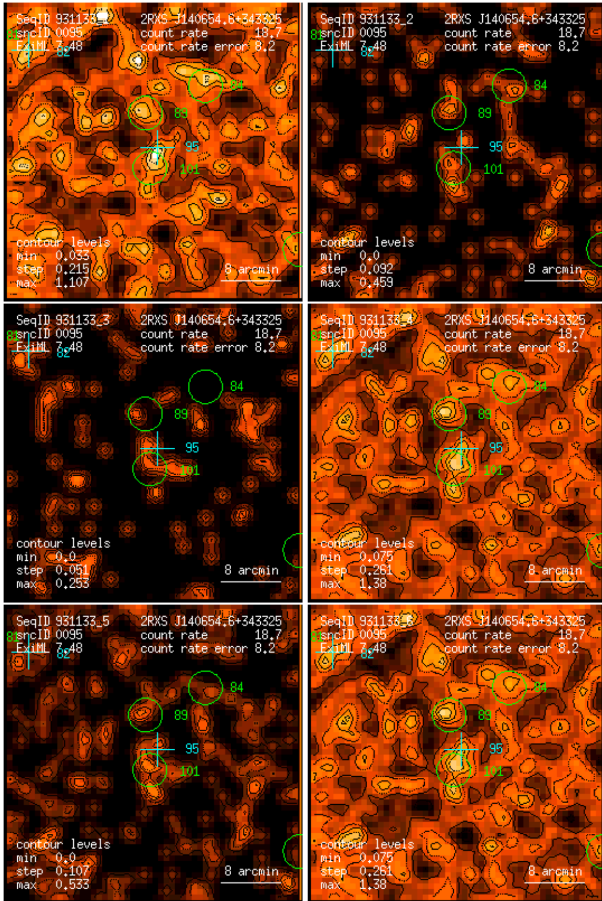
Figure 95: RASS 931133: detection 0095: band rate images, Gaussian filter: (1) PSPC channels 11 – 41, (2) 52 – 90, (3) 91 – 201, (4) 11 – 235, (5) 52 – 201, (6) 11 – 201. Broad band rates in counts/ks. Band rate contour levels in counts/ks/arcmin 2 .
