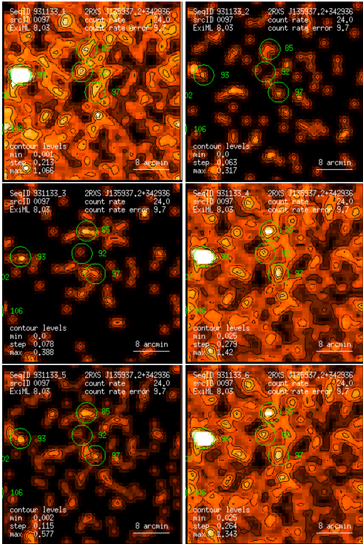
Figure 97: RASS 931133: detection 0097: band rate images, Gaussian filter: (1) PSPC channels 11 – 41, (2) 52 – 90, (3) 91 – 201, (4) 11 – 235, (5) 52 – 201, (6) 11 – 201. Broad band rates in counts/ks. Band rate contour levels in counts/ks/arcmin 2 .
