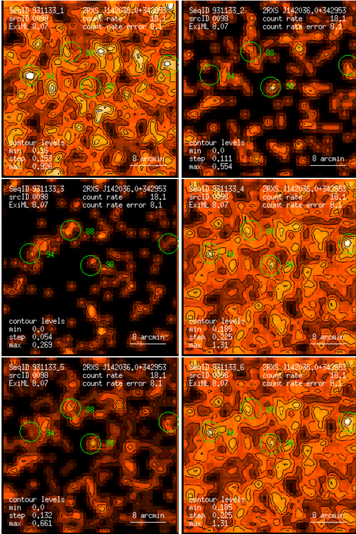
Figure 98: RASS 931133: detection 0098: band rate images, Gaussian filter: (1) PSPC channels 11 – 41, (2) 52 – 90, (3) 91 – 201, (4) 11 – 235, (5) 52 – 201, (6) 11 – 201. Broad band rates in counts/ks. Band rate contour levels in counts/ks/arcmin 2 .
