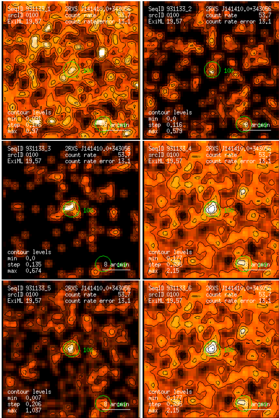
Figure 100: RASS 931133: detection 0100: band rate images, Gaussian filter: (1) PSPC channels 11 – 41, (2) 52 – 90, (3) 91 – 201, (4) 11 – 235, (5) 52 – 201, (6) 11 – 201. Broad band rates in counts/ks. Band rate contour levels in counts/ks/arcmin 2 .
