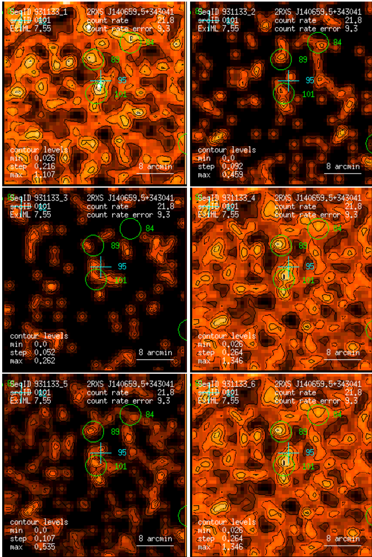
Figure 101: RASS 931133: detection 0101: band rate images, Gaussian filter: (1) PSPC channels 11 – 41, (2) 52 – 90, (3) 91 – 201, (4) 11 – 235, (5) 52 – 201, (6) 11 – 201. Broad band rates in counts/ks. Band rate contour levels in counts/ks/arcmin 2 .
