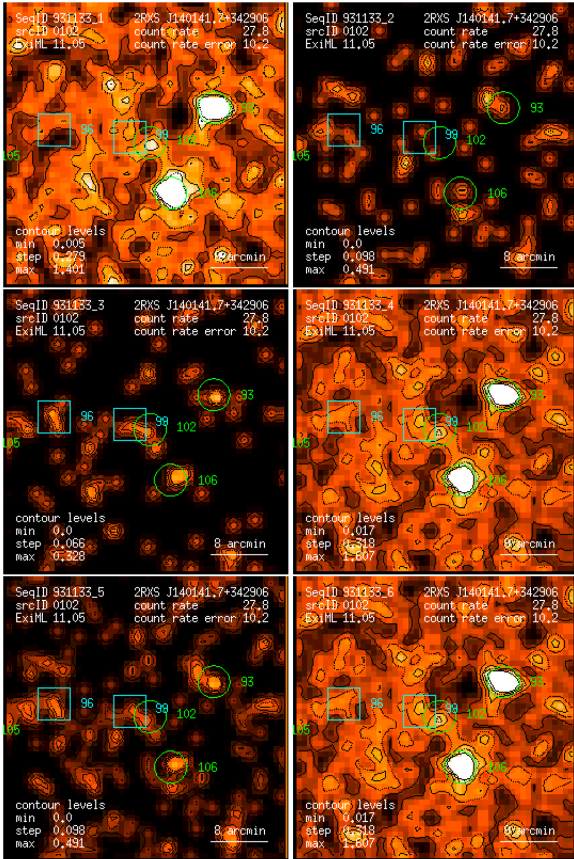
Figure 102: RASS 931133: detection 0102: band rate images, Gaussian filter: (1) PSPC channels 11 – 41, (2) 52 – 90, (3) 91 – 201, (4) 11 – 235, (5) 52 – 201, (6) 11 – 201. Broad band rates in counts/ks. Band rate contour levels in counts/ks/arcmin 2 .
