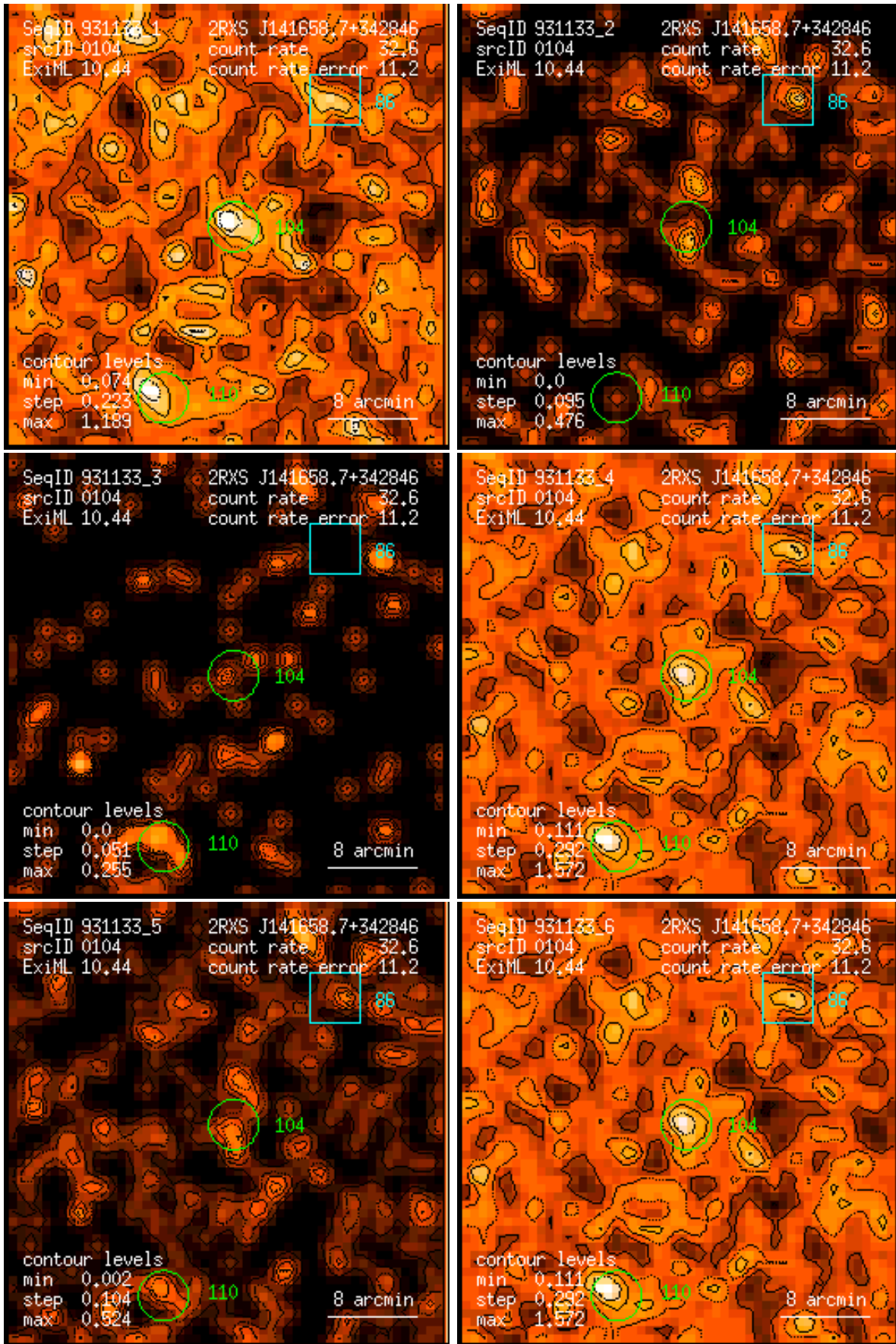
Figure 104: RASS 931133: detection 0104: band rate images, Gaussian filter: (1) PSPC channels 11 – 41, (2) 52 – 90, (3) 91 – 201, (4) 11 – 235, (5) 52 – 201, (6) 11 – 201. Broad band rates in counts/ks. Band rate contour levels in counts/ks/arcmin 2 .
