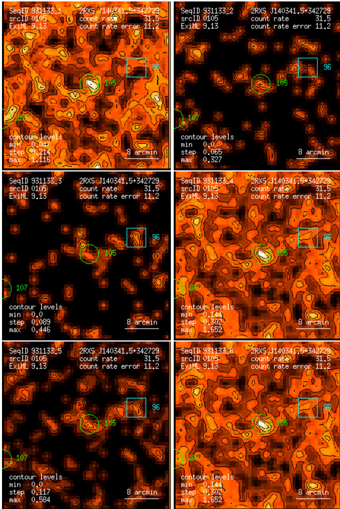
Figure 105: RASS 931133: detection 0105: band rate images, Gaussian filter: (1) PSPC channels 11 – 41, (2) 52 – 90, (3) 91 – 201, (4) 11 – 235, (5) 52 – 201, (6) 11 – 201. Broad band rates in counts/ks. Band rate contour levels in counts/ks/arcmin 2 .
