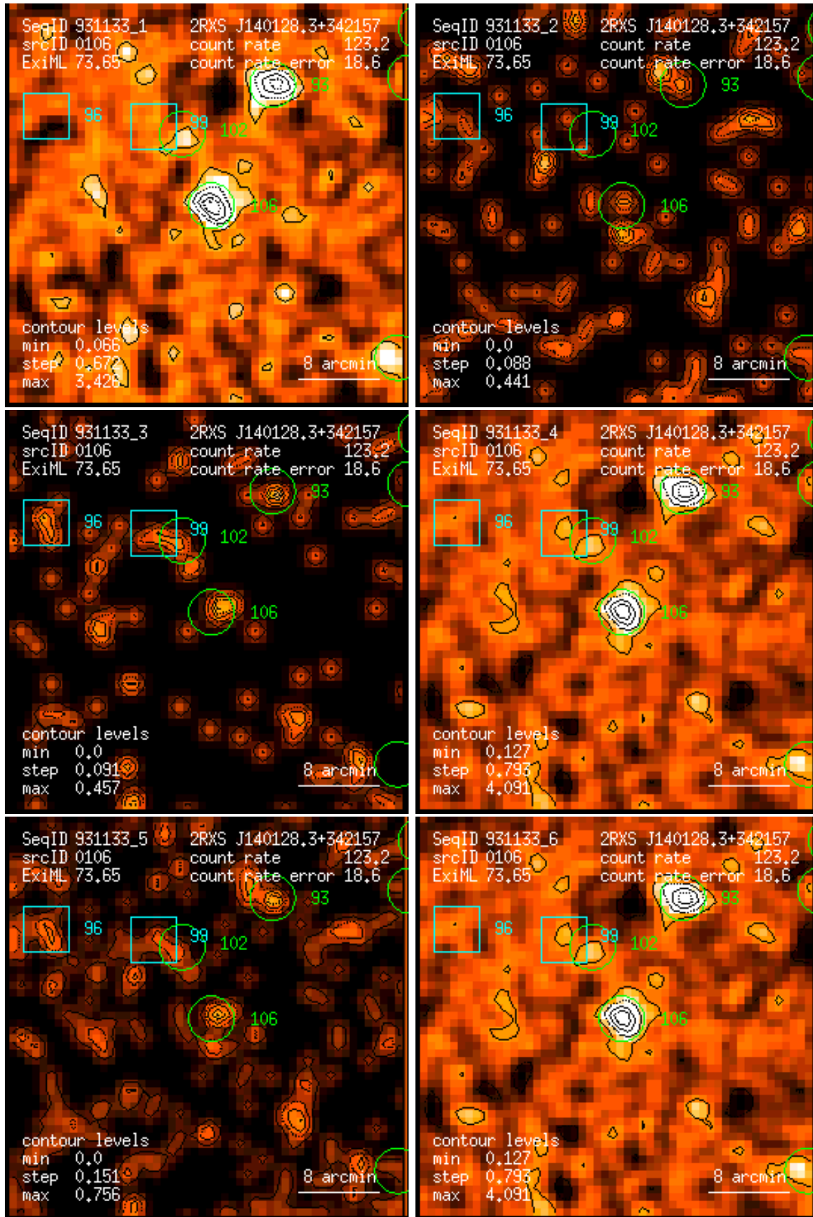
Figure 106: RASS 931133: detection 0106: band rate images, Gaussian filter: (1) PSPC channels 11 – 41, (2) 52 – 90, (3) 91 – 201, (4) 11 – 235, (5) 52 – 201, (6) 11 – 201. Broad band rates in counts/ks. Band rate contour levels in counts/ks/arcmin 2 .
