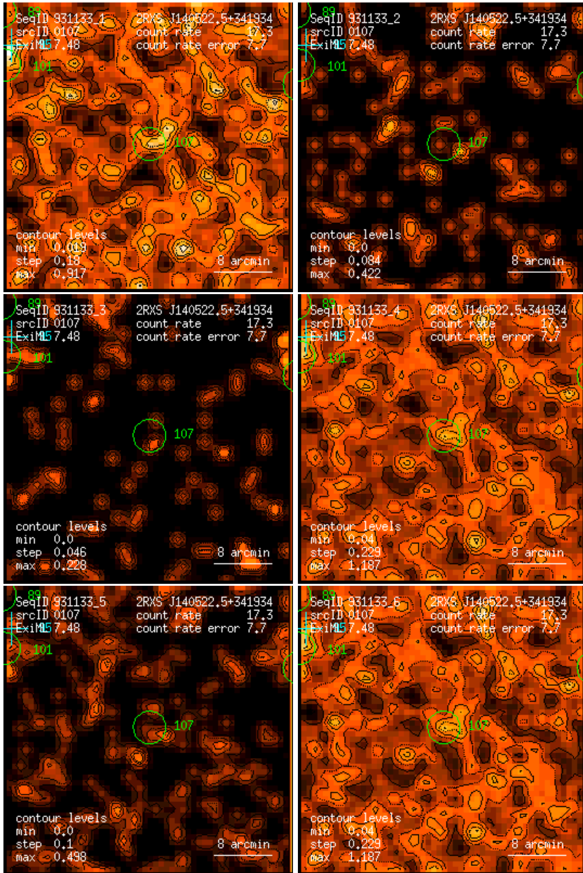
Figure 107: RASS 931133: detection 0107: band rate images, Gaussian filter: (1) PSPC channels 11 – 41, (2) 52 – 90, (3) 91 – 201, (4) 11 – 235, (5) 52 – 201, (6) 11 – 201. Broad band rates in counts/ks. Band rate contour levels in counts/ks/arcmin 2 .
