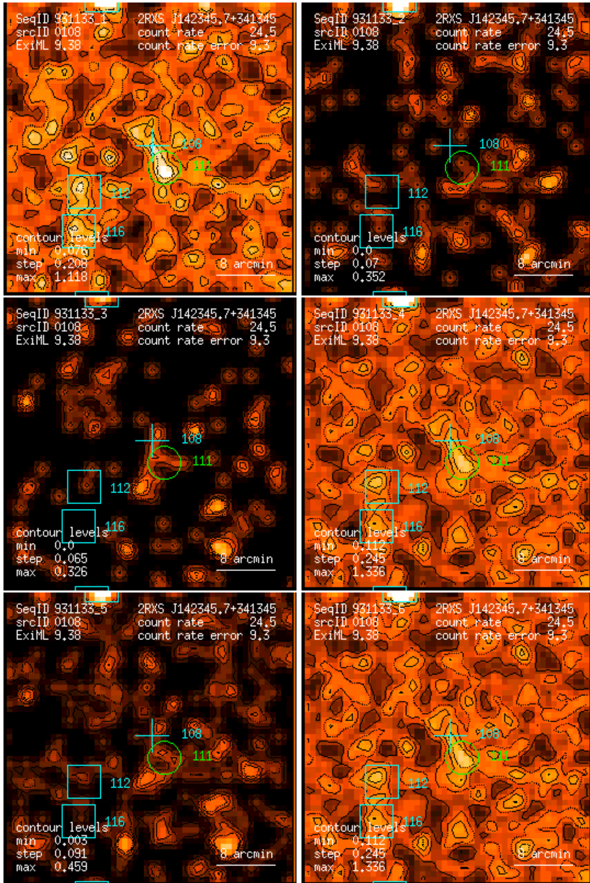
Figure 108: RASS 931133: detection 0108: band rate images, Gaussian filter: (1) PSPC channels 11 – 41, (2) 52 – 90, (3) 91 – 201, (4) 11 – 235, (5) 52 – 201, (6) 11 – 201. Broad band rates in counts/ks. Band rate contour levels in counts/ks/arcmin 2 .
