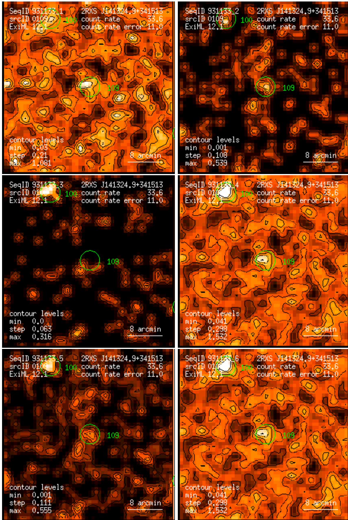
Figure 109: RASS 931133: detection 0109: band rate images, Gaussian filter: (1) PSPC channels 11 – 41, (2) 52 – 90, (3) 91 – 201, (4) 11 – 235, (5) 52 – 201, (6) 11 – 201. Broad band rates in counts/ks. Band rate contour levels in counts/ks/arcmin 2 .
