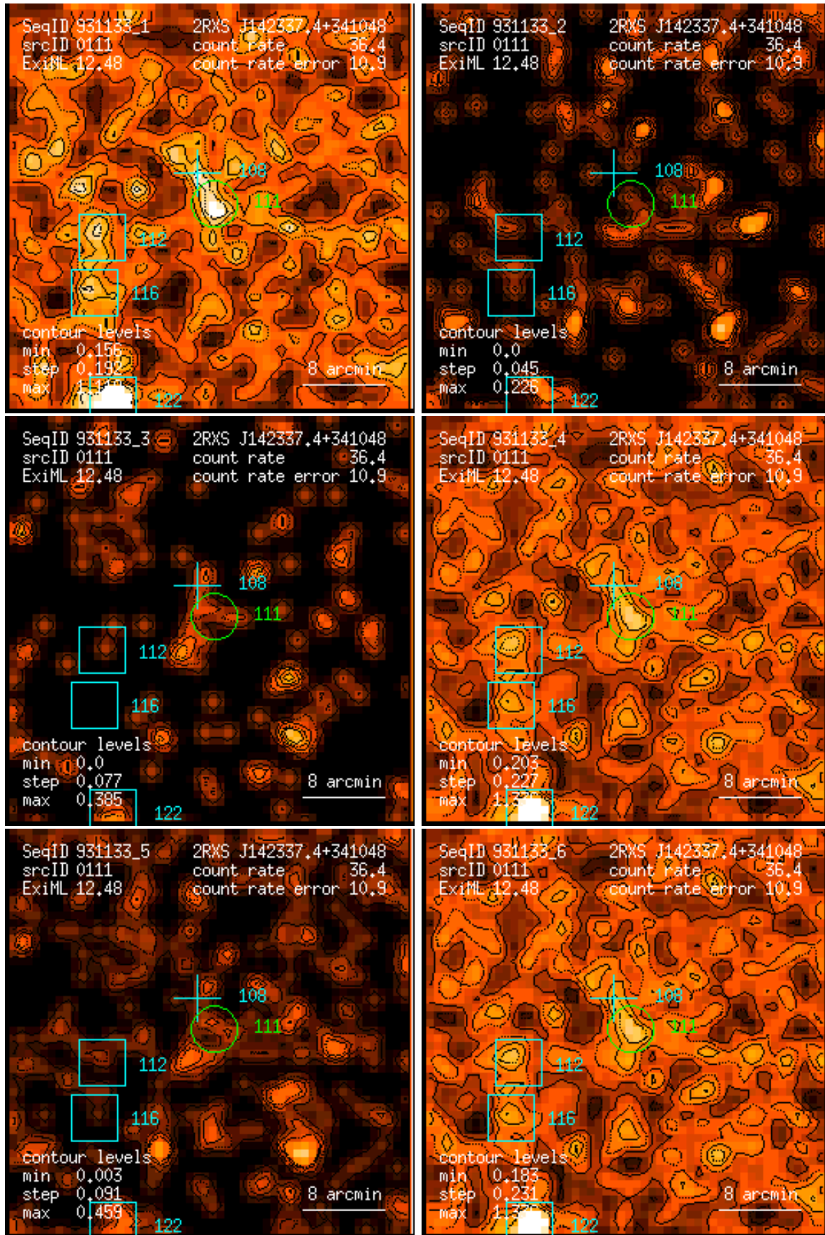
Figure 111: RASS 931133: detection 0111: band rate images, Gaussian filter: (1) PSPC channels 11 – 41, (2) 52 – 90, (3) 91 – 201, (4) 11 – 235, (5) 52 – 201, (6) 11 – 201. Broad band rates in counts/ks. Band rate contour levels in counts/ks/arcmin 2 .
