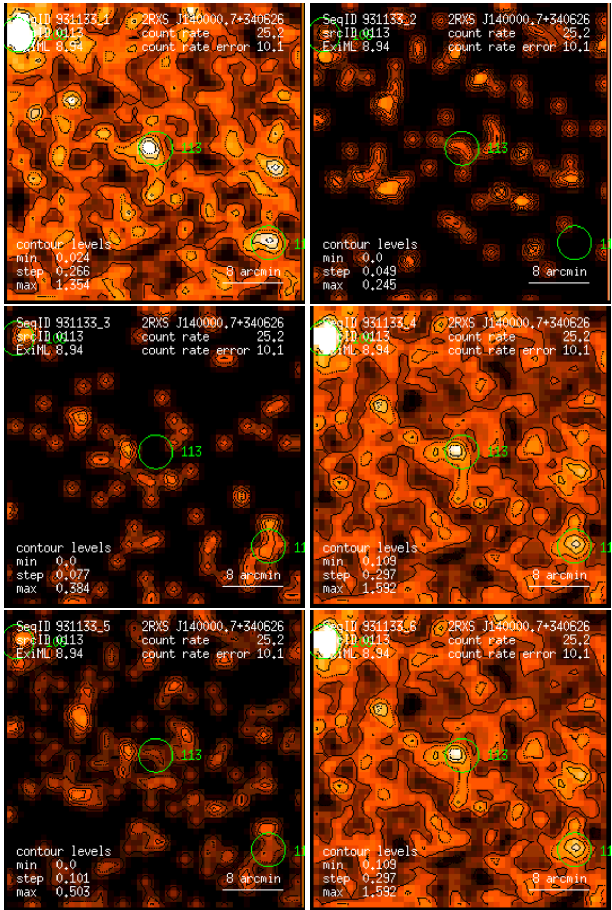
Figure 113: RASS 931133: detection 0113: band rate images, Gaussian filter: (1) PSPC channels 11 – 41, (2) 52 – 90, (3) 91 – 201, (4) 11 – 235, (5) 52 – 201, (6) 11 – 201. Broad band rates in counts/ks. Band rate contour levels in counts/ks/arcmin 2 .
