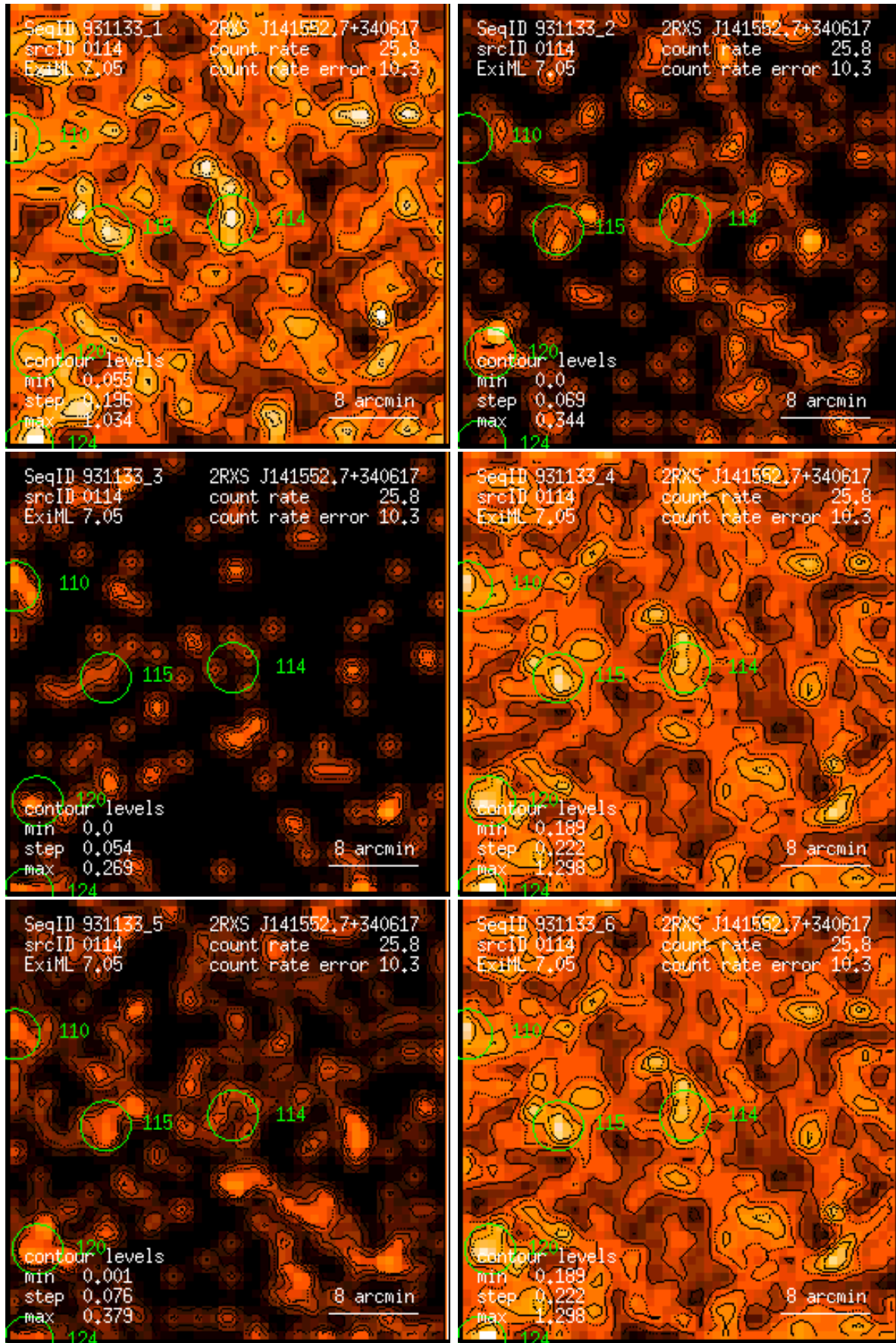
Figure 114: RASS 931133: detection 0114: band rate images, Gaussian filter: (1) PSPC channels 11 – 41, (2) 52 – 90, (3) 91 – 201, (4) 11 – 235, (5) 52 – 201, (6) 11 – 201. Broad band rates in counts/ks. Band rate contour levels in counts/ks/arcmin 2 .
