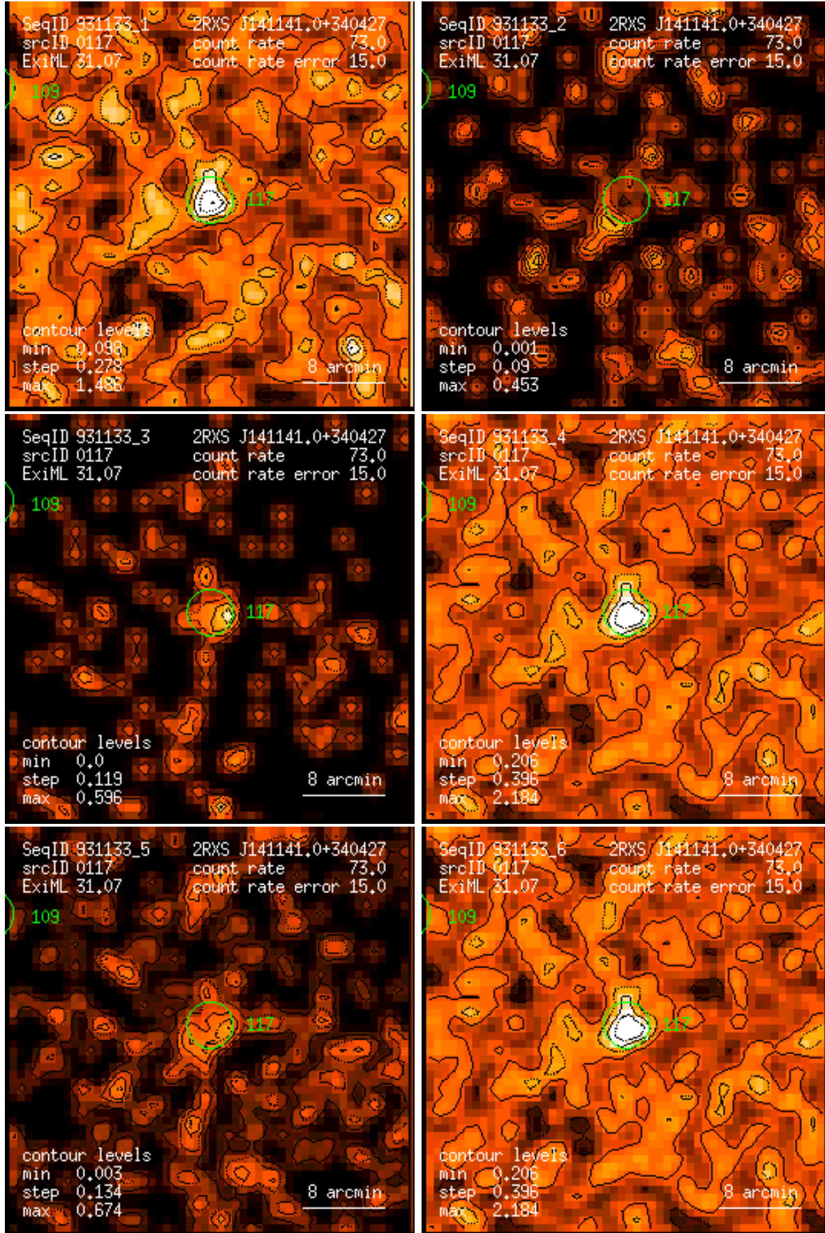
Figure 117: RASS 931133: detection 0117: band rate images, Gaussian filter: (1) PSPC channels 11 – 41, (2) 52 – 90, (3) 91 – 201, (4) 11 – 235, (5) 52 – 201, (6) 11 – 201. Broad band rates in counts/ks. Band rate contour levels in counts/ks/arcmin 2 .
