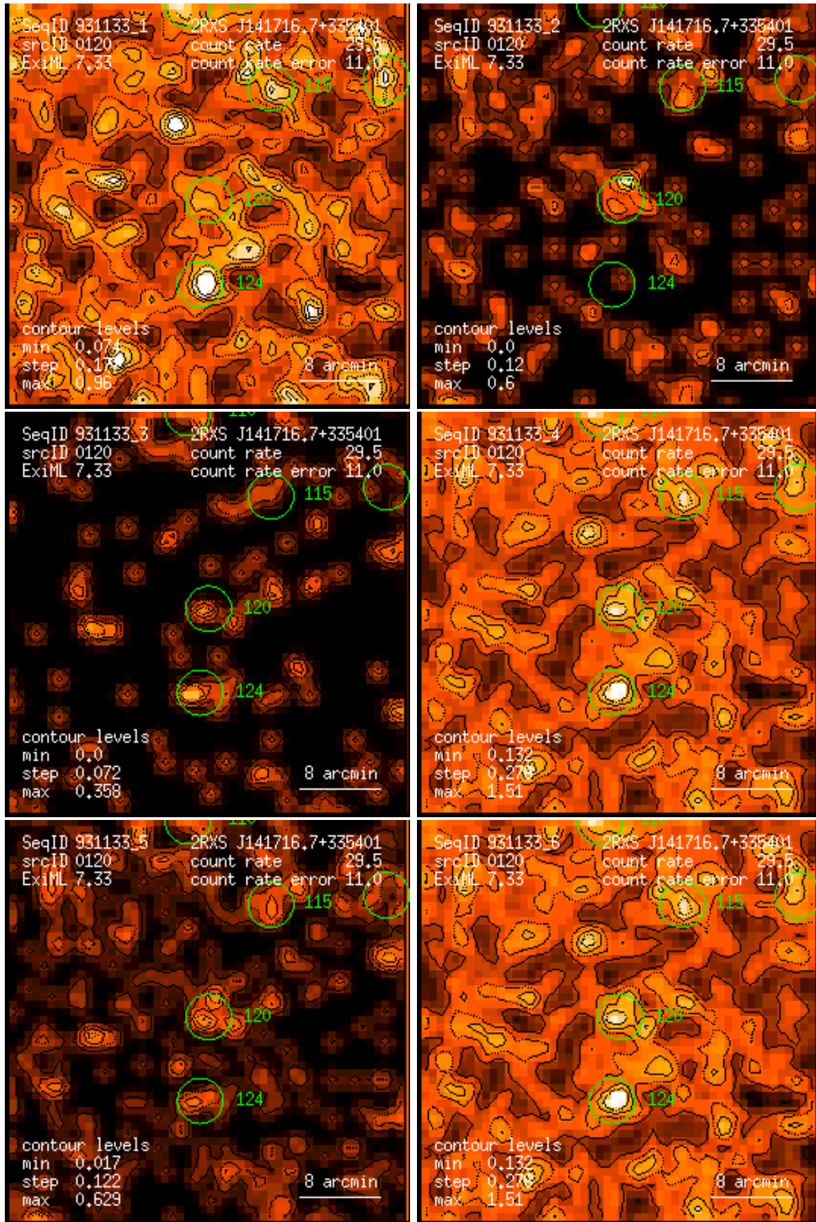
Figure 120: RASS 931133: detection 0120: band rate images, Gaussian filter: (1) PSPC channels 11 – 41, (2) 52 – 90, (3) 91 – 201, (4) 11 – 235, (5) 52 – 201, (6) 11 – 201. Broad band rates in counts/ks. Band rate contour levels in counts/ks/arcmin 2 .
