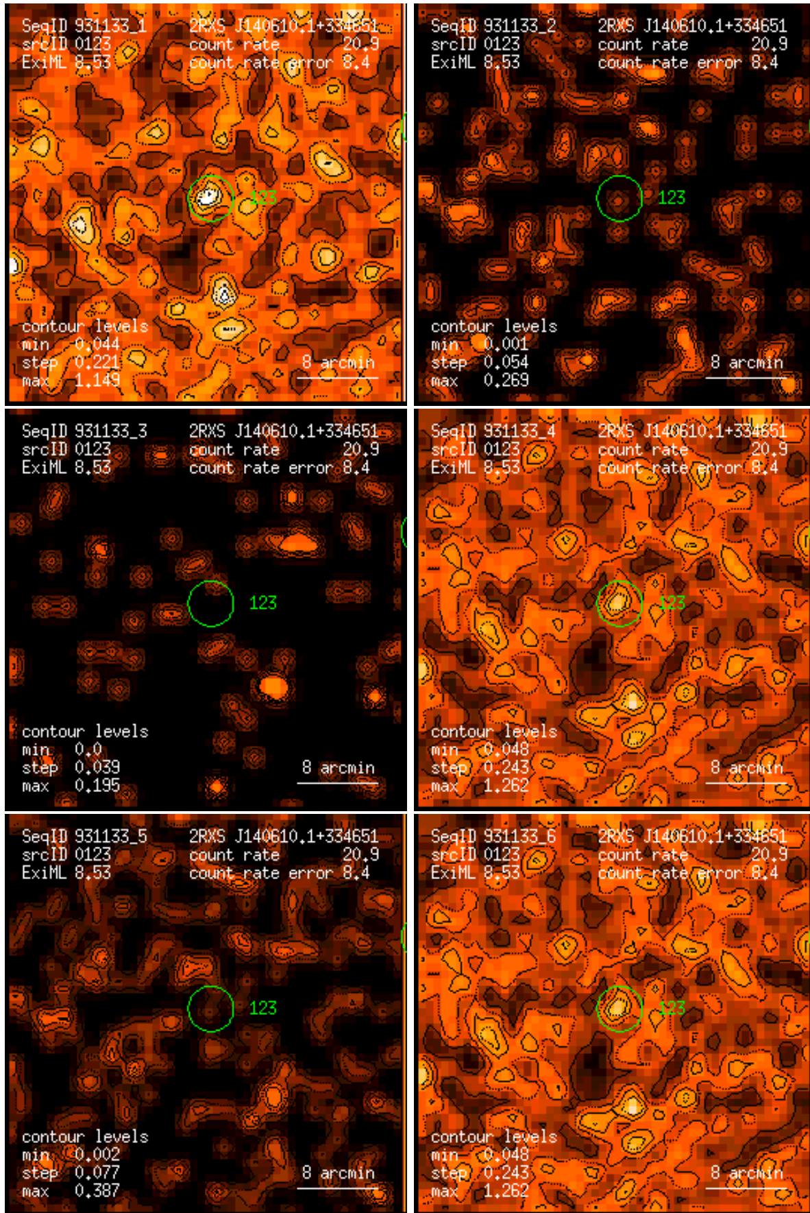
Figure 123: RASS 931133: detection 0123: band rate images, Gaussian filter: (1) PSPC channels 11 – 41, (2) 52 – 90, (3) 91 – 201, (4) 11 – 235, (5) 52 – 201, (6) 11 – 201. Broad band rates in counts/ks. Band rate contour levels in counts/ks/arcmin 2 .
