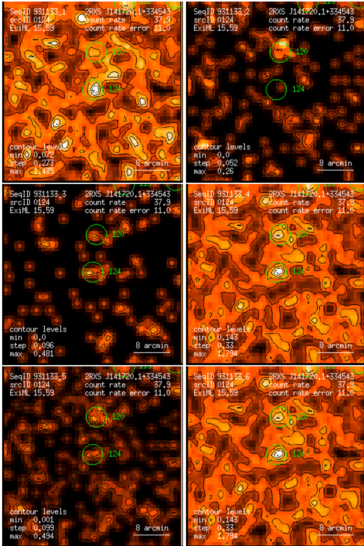
Figure 124: RASS 931133: detection 0124: band rate images, Gaussian filter: (1) PSPC channels 11 – 41, (2) 52 – 90, (3) 91 – 201, (4) 11 – 235, (5) 52 – 201, (6) 11 – 201. Broad band rates in counts/ks. Band rate contour levels in counts/ks/arcmin 2 .
