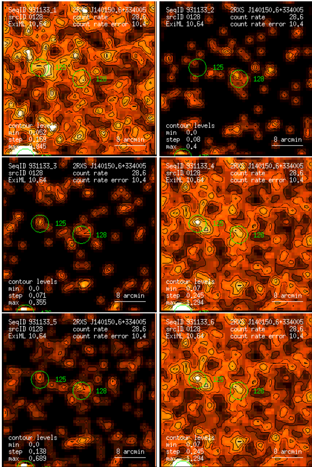
Figure 128: RASS 931133: detection 0128: band rate images, Gaussian filter: (1) PSPC channels 11 – 41, (2) 52 – 90, (3) 91 – 201, (4) 11 – 235, (5) 52 – 201, (6) 11 – 201. Broad band rates in counts/ks. Band rate contour levels in counts/ks/arcmin 2 .
