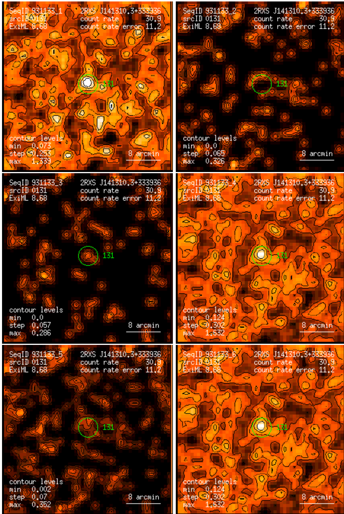
Figure 131: RASS 931133: detection 0131: band rate images, Gaussian filter: (1) PSPC channels 11 – 41, (2) 52 – 90, (3) 91 – 201, (4) 11 – 235, (5) 52 – 201, (6) 11 – 201. Broad band rates in counts/ks. Band rate contour levels in counts/ks/arcmin 2 .
