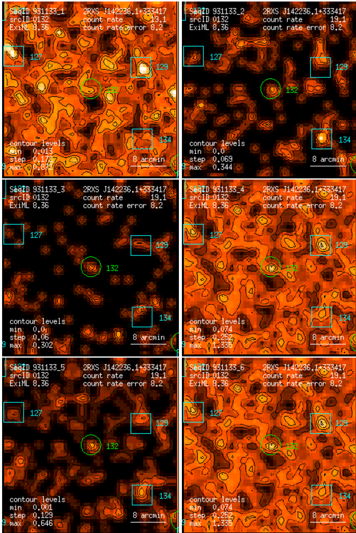
Figure 132: RASS 931133: detection 0132: band rate images, Gaussian filter: (1) PSPC channels 11 – 41, (2) 52 – 90, (3) 91 – 201, (4) 11 – 235, (5) 52 – 201, (6) 11 – 201. Broad band rates in counts/ks. Band rate contour levels in counts/ks/arcmin 2 .
