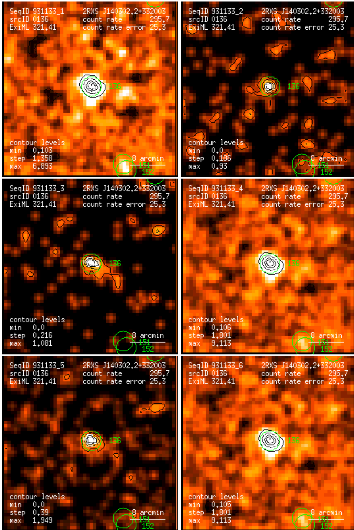
Figure 136: RASS 931133: detection 0136: band rate images, Gaussian filter: (1) PSPC channels 11 – 41, (2) 52 – 90, (3) 91 – 201, (4) 11 – 235, (5) 52 – 201, (6) 11 – 201. Broad band rates in counts/ks. Band rate contour levels in counts/ks/arcmin 2 .
