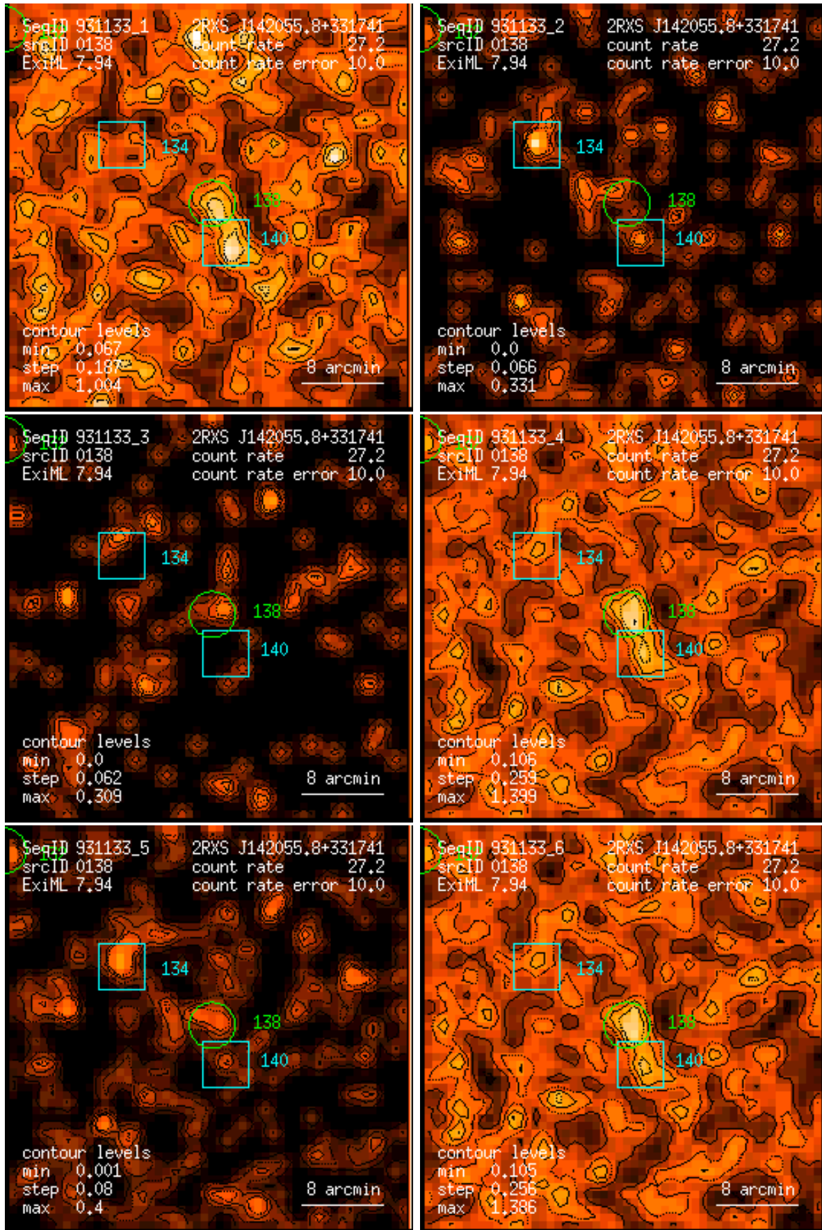
Figure 138: RASS 931133: detection 0138: band rate images, Gaussian filter: (1) PSPC channels 11 – 41, (2) 52 – 90, (3) 91 – 201, (4) 11 – 235, (5) 52 – 201, (6) 11 – 201. Broad band rates in counts/ks. Band rate contour levels in counts/ks/arcmin 2 .
