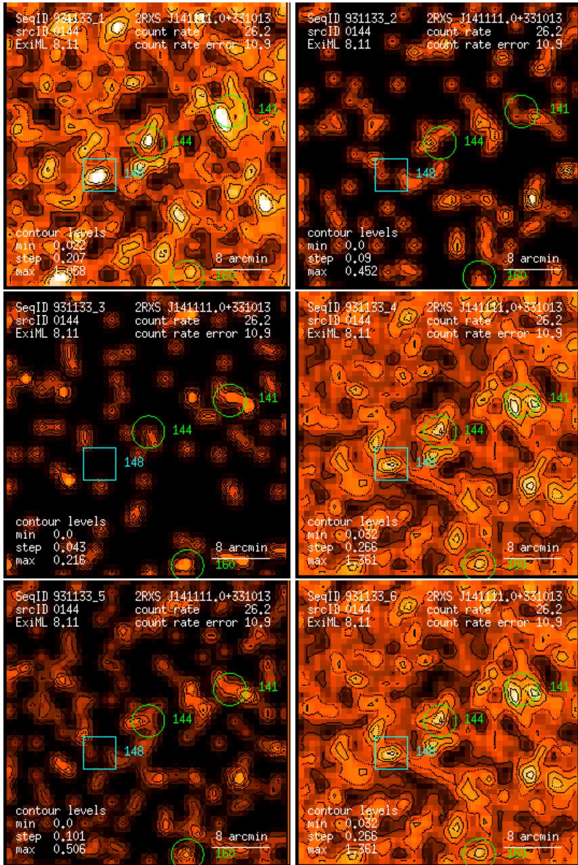
Figure 144: RASS 931133: detection 0144: band rate images, Gaussian filter: (1) PSPC channels 11 – 41, (2) 52 – 90, (3) 91 – 201, (4) 11 – 235, (5) 52 – 201, (6) 11 – 201. Broad band rates in counts/ks. Band rate contour levels in counts/ks/arcmin 2 .
