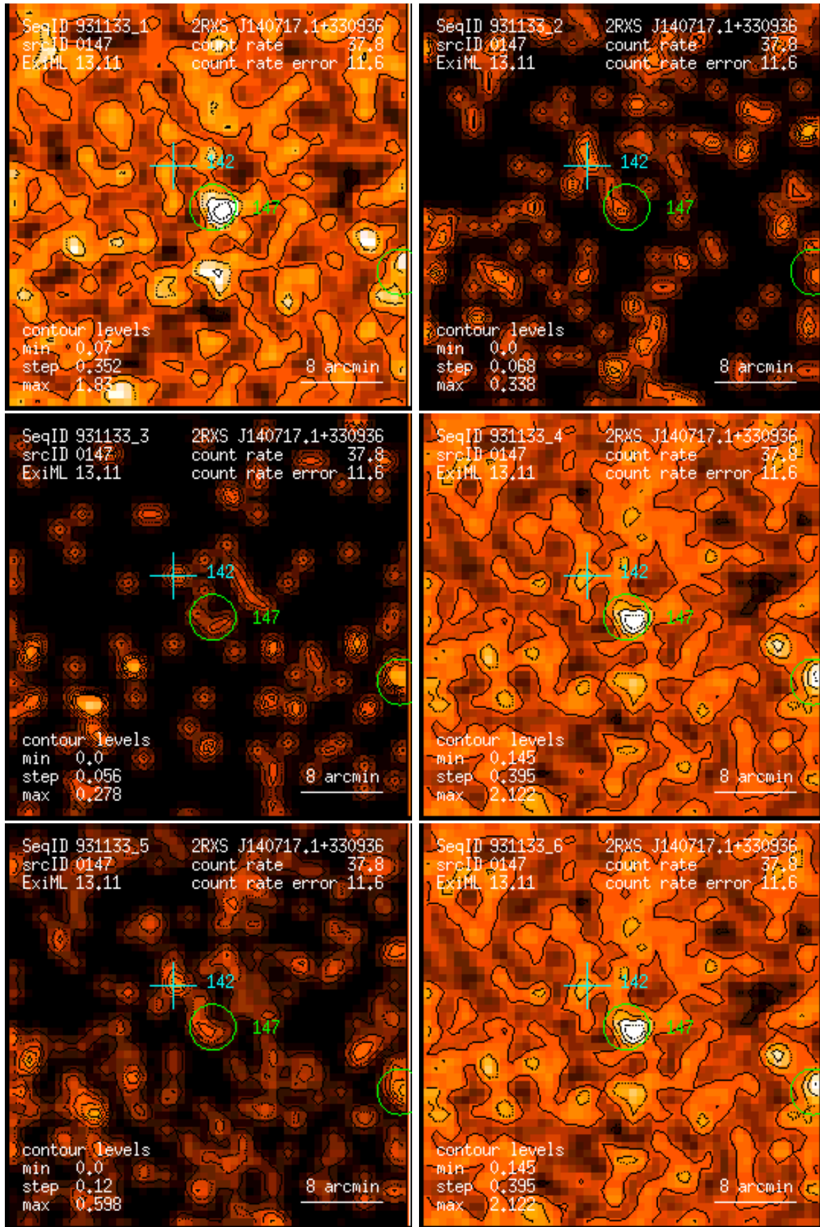
Figure 147: RASS 931133: detection 0147: band rate images, Gaussian filter: (1) PSPC channels 11 – 41, (2) 52 – 90, (3) 91 – 201, (4) 11 – 235, (5) 52 – 201, (6) 11 – 201. Broad band rates in counts/ks. Band rate contour levels in counts/ks/arcmin 2 .
