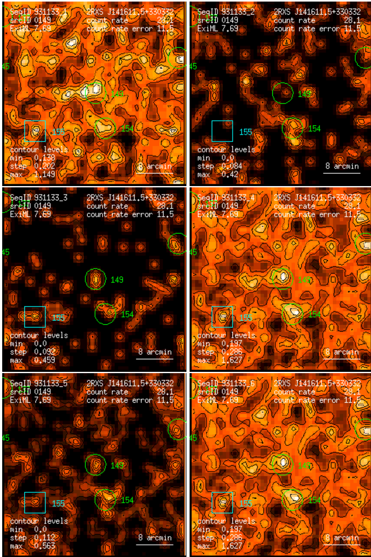
Figure 149: RASS 931133: detection 0149: band rate images, Gaussian filter: (1) PSPC channels 11 – 41, (2) 52 – 90, (3) 91 – 201, (4) 11 – 235, (5) 52 – 201, (6) 11 – 201. Broad band rates in counts/ks. Band rate contour levels in counts/ks/arcmin 2 .
