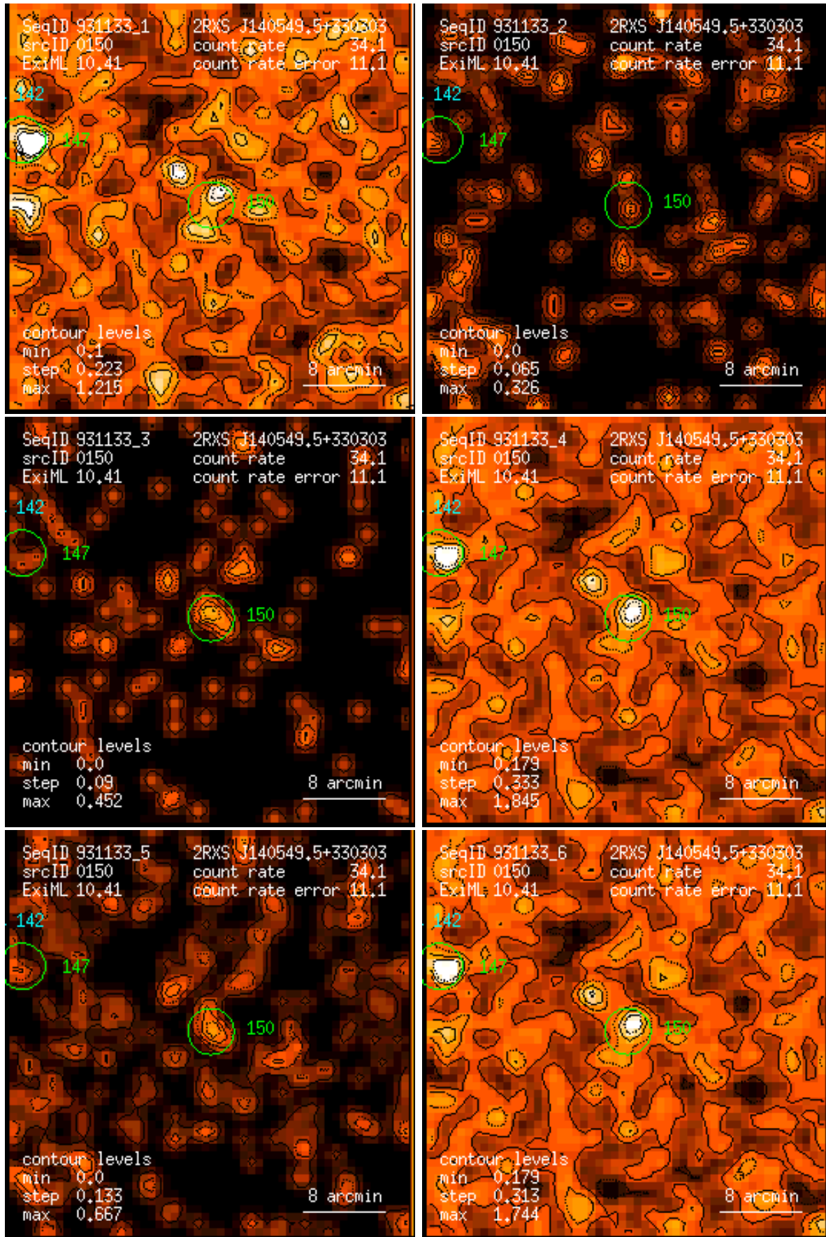
Figure 150: RASS 931133: detection 0150: band rate images, Gaussian filter: (1) PSPC channels 11 – 41, (2) 52 – 90, (3) 91 – 201, (4) 11 – 235, (5) 52 – 201, (6) 11 – 201. Broad band rates in counts/ks. Band rate contour levels in counts/ks/arcmin 2 .
