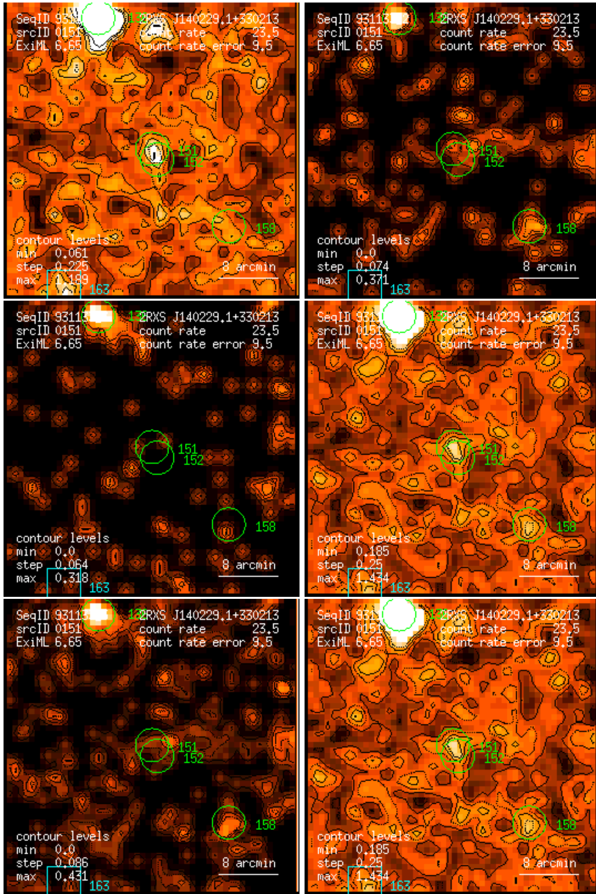
Figure 151: RASS 931133: detection 0151: band rate images, Gaussian filter: (1) PSPC channels 11 – 41, (2) 52 – 90, (3) 91 – 201, (4) 11 – 235, (5) 52 – 201, (6) 11 – 201. Broad band rates in counts/ks. Band rate contour levels in counts/ks/arcmin 2 .
